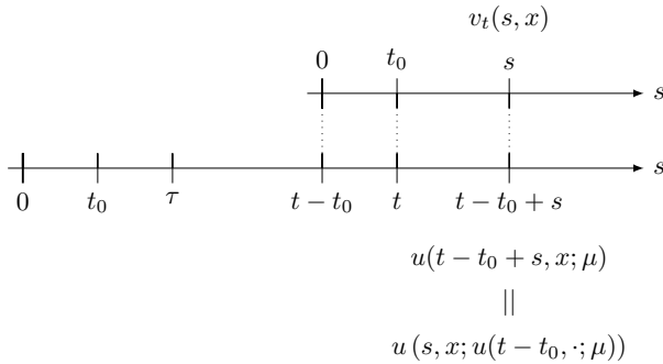
Fig. 3 An illustration for the restarted SHE in (44).
