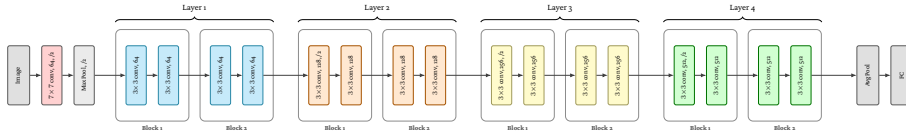
Figure 2.5: Detailed ResNet-18 structure with BasicBlock containers. Each residual stage contains two BasicBlocks, and each BasicBlock contains two convolution operations. The first block of layers 2–4 includes a projection shortcut for downsampling.
