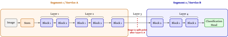
Figure 2.6: Block-level two-segment decomposition used in Stage L2. The refined split point is placed inside layer 3, after the first residual block. Segment 1 executes the stem through layer 3 . 0; Segment 2 receives the intermediate activation tensor and executes layer 3 . 1 through the classification head.
