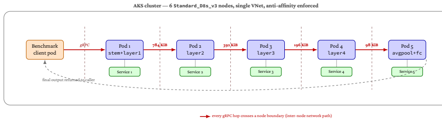
Figure 2.9: Stage C (multi-node) AKS placement of chain_5svc. Each chain segment lands on a distinct cluster node; the benchmark client pod lands on a sixth dedicated node. Every gRPC hop therefore crosses a node boundary, in contrast to the same-node layout used for Stage K and Stage C (fig. 2.8).
