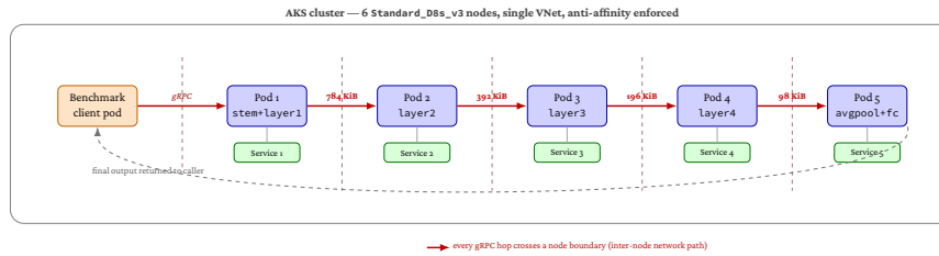
Figure 2.9: Stage C (multi-node) AKS placement of chain_5svc . Each chain segment lands on a distinct cluster node; the benchmark client pod lands on a sixth dedicated node. Every gRPC hop therefore crosses a node boundary, in contrast to the same-node layout used for Stage K and Stage C (fig. 2.8).
