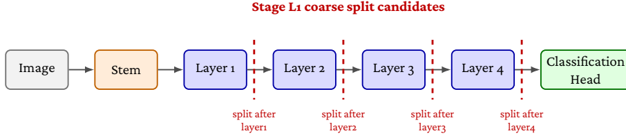
Figure 2.3: Coarse ResNet-18 partition boundaries evaluated in Stage L1. The stem and classification head are collapsed into single blocks, while the four residual stages are shown as the candidate split locations.
