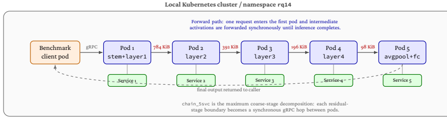
Figure 2.8: Kubernetes pod and service placement for the Stage K five-service chain. The benchmark client and all inference pods are placed on the same Kubernetes node, while each model segment is exposed through a Kubernetes Service and communicates using synchronous gRPC forwarding. The labels above the arrows show the activation-transfer size at each coarse ResNet-18 boundary.
