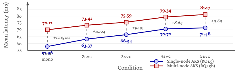
Figure 5.6: RQ1.5b multi-node penalty per condition. Same SKU (Standard_D8s_v3), same region (swedencentral), same day; the only difference is single-node colocation versus multi_node_anti_affinity placement. The penalty is dominated by the first inter-node hop (the client→service-1 transfer of the 600 KiB input tensor over the VNet); per-condition deltas in the chained conditions stay in the narrow band of 8.6–10.0 ms.
