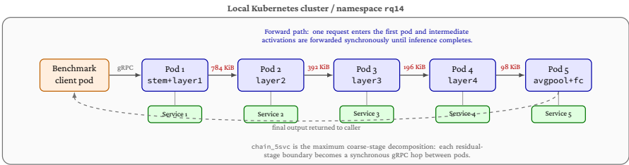
Figure 2.9: Kubernetes pod and service placement for the RQ1.4 five-service chain. The benchmark client and all inference pods are placed on the same Kubernetes node, while each model segment is exposed through a Kubernetes Service and communicates using synchronous gRPC forwarding. The labels above the arrows show the activation-transfer size at each coarse ResNet-18 boundary.
