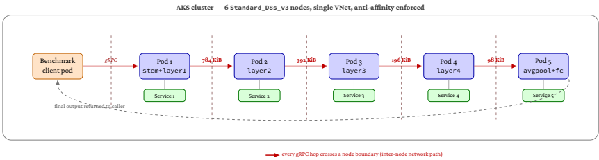
Figure 2.8: RQ1.4b / RQ1.5b multi-node placement of chain_5svc. Each chain segment lands on a distinct cluster node; the benchmark client pod lands on a sixth dedicated node. Every gRPC hop therefore crosses a node boundary, in contrast to the same-figure single-node layout used for RQ1.4 and RQ1.5 (fig. 2.9).
