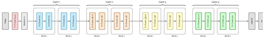
Figure 2.7: Detailed ResNet-18 structure with BasicBlock containers. Each residual stage contains two BasicBlocks, and each BasicBlock contains two convolution operations. The first block of layers 2–4 includes a projection shortcut for downsampling.
