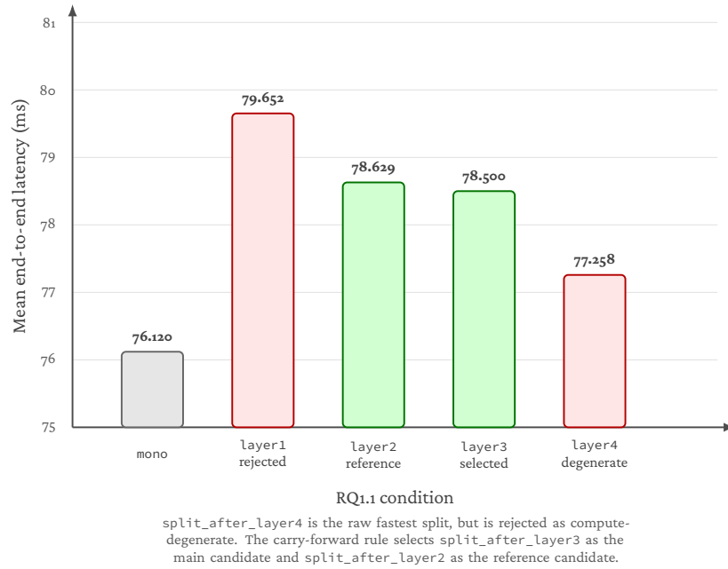
Figure 5.1: RQ1.1 coarse split latency results under controlled local execution. Although split_after_layer4 has the lowest mean latency among split configurations, it is rejected by the compute-degeneracy rule. The selected carry-forward candidates are split_after_layer3 and split_after_layer2 .
