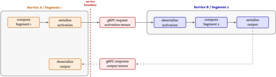
Figure 2.7: Runtime cost components introduced by a two-service inference boundary. In addition to the model computation on each side of the split, the intermediate activation must be serialized, transferred through gRPC, deserialized by the downstream service, and followed by response serialization and reconstruction. The boundary-crossing interval therefore includes serialization, RPC transport, remote execution, and response reconstruction.
