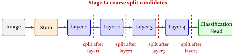
Figure 2.3: Coarse ResNet-18 partition boundaries evaluated in Stage L1. The stem and classification head are collapsed into single blocks, while the four residual stages are shown as the candidate split locations.
