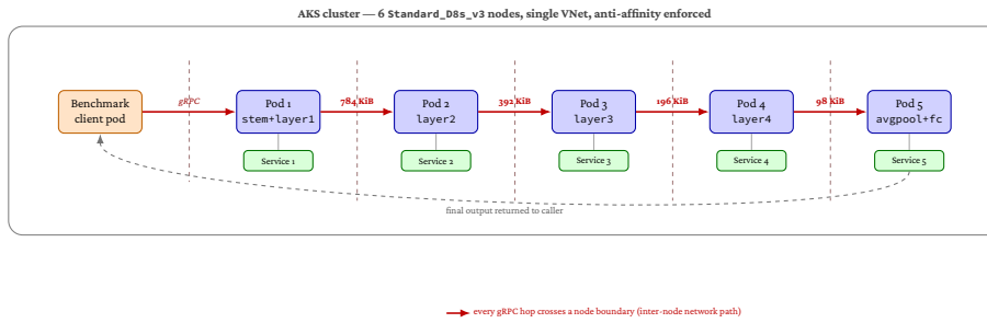
Figure 2.9: Stage C (multi-node) AKS placement of chain_5svc . Each chain segment lands on a distinct cluster node; the benchmark client pod lands on a sixth dedicated node. Every gRPC hop therefore crosses a node boundary, in contrast to the same-node layout used for Stage K and Stage C (fig. 2.8).
