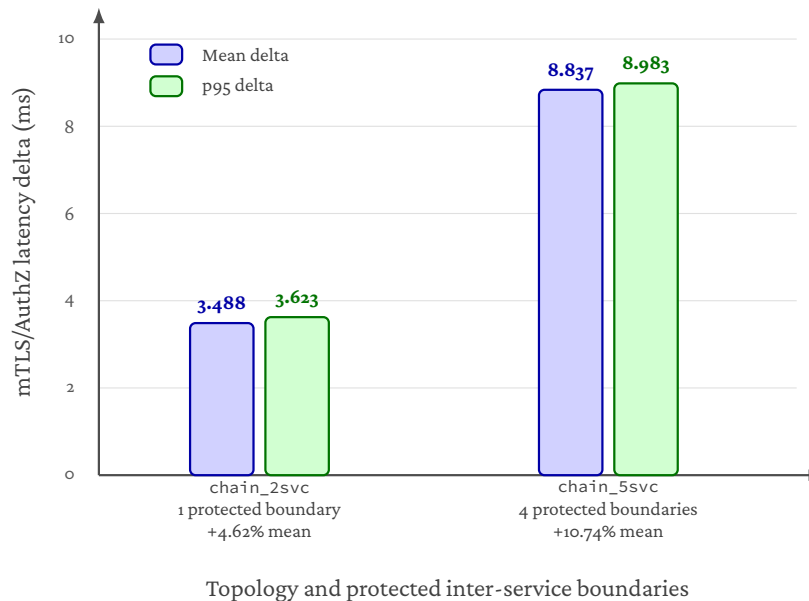
Figure 5.7: Stage H1 mTLS/AuthZ latency overhead for the primary and stress AKS chains. Mean and p95 deltas are computed within the paired plain/mTLS design. The stress topology contains four protected inter-service boundaries, so the larger overhead visualises the observed stress-case sensitivity of sidecar-mediated communication hardening.
