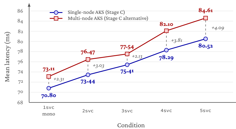
Figure 5.6: Stage C (multi-node) inter-node penalty per condition. Same SKU (Standard_D8s_v3), same region (swedencentral); the intentional experimental contrast is single-node colocation versus multi_node_anti_affinity placement. The figure is manually rendered from the same frozen summary artefacts as table 5.14. Per-condition deltas range from 2.131 ms (chain_3svc) to 4.086 ms (chain_5svc), and the monolithic-baseline penalty is 2.305 ms.
