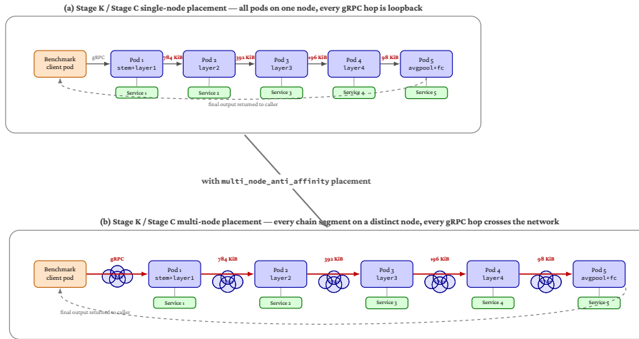
Figure 5.5: Same chain, two topologies. (a) Stage K / Stage C single-node (base-case) placement: all six pods on one node, every gRPC hop is loopback. (b) Stage K / Stage C multi-node (alternative) placement: each chain segment lands on a distinct cluster node and the client lands on a sixth dedicated node, so every gRPC hop crosses the Azure VNet. The chain itself is identical between the two panels; only the pod-to-node assignment changes.
