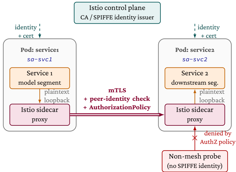
Figure 2.9: Service identity, mTLS, and authorization between two inference services. The Istio control plane mints SPIFFE workload identities and certificates for each sidecar (dashed teal arrows). The protected inter-pod hop carries mTLS plus an identity-bound AuthorizationPolicy check between the workload identities sa-svc1 and sa-svc2 (purple double arrow), while application-to-sidecar traffic inside each pod stays plaintext (orange arrows). A non-mesh probe that lacks a SPIFFE identity is rejected at the receiving sidecar by the same authorization policy (red arrow with cross).
