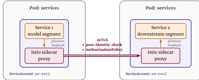
Figure 2.10: Communication-level hardening between two inference services. Each pod runs an Istio sidecar proxy that terminates TLS at the pod boundary. The inter-pod hop carries mTLS plus an identity-bound AuthorizationPolicy check between the workload identities sa-svc1 and sa-svc2 . Application-to-sidecar traffic inside each pod remains plaintext.
