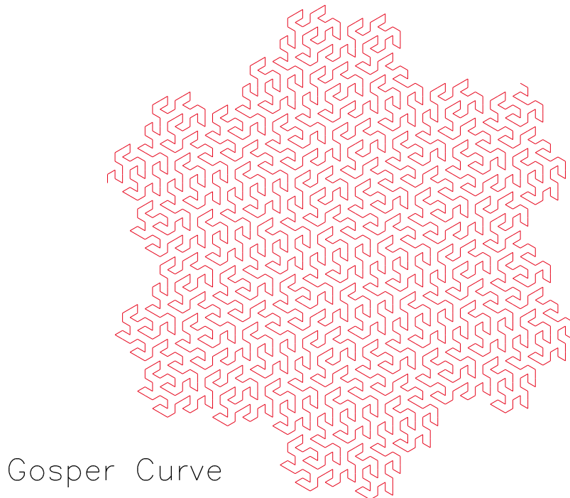
Figure 48: A Gosper Flowsnake curve (4 iterations)
