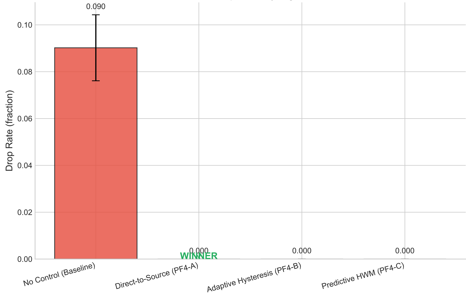
Packet Drop Rate by Algorithm
