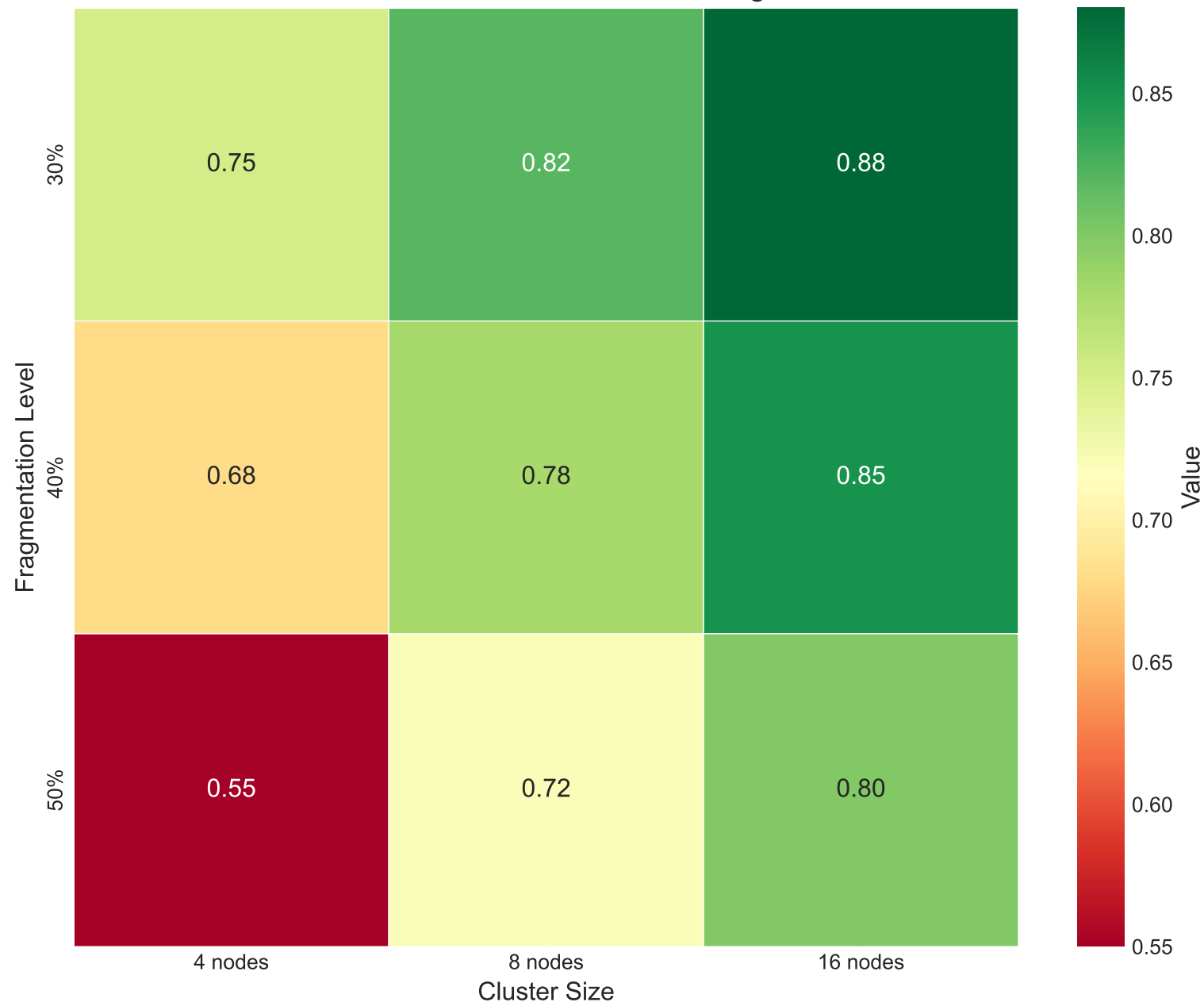
Cluster Utilization: Balanced Borrow Algorithm
