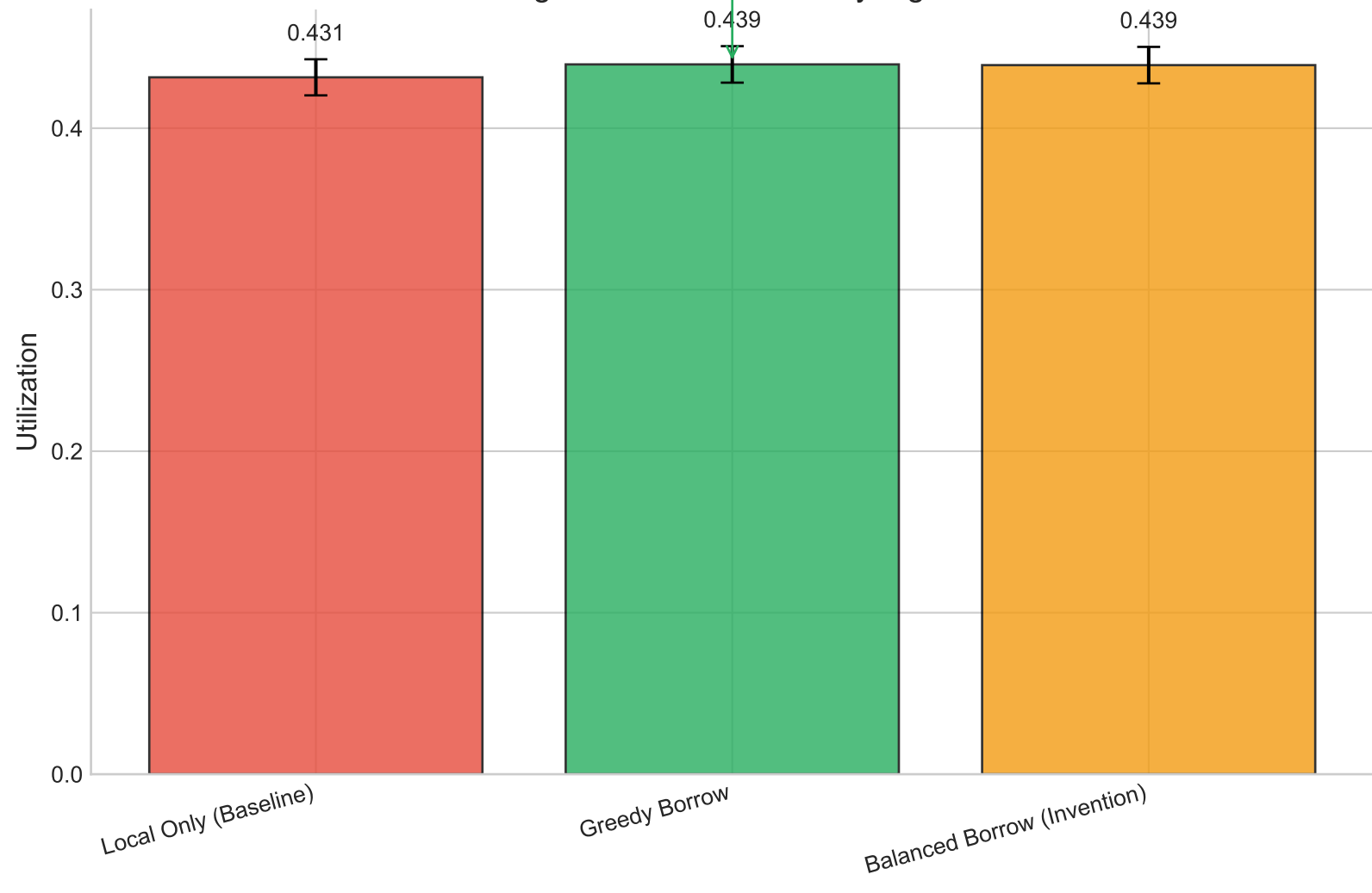
Average Cluster Utilization by Algorithm
