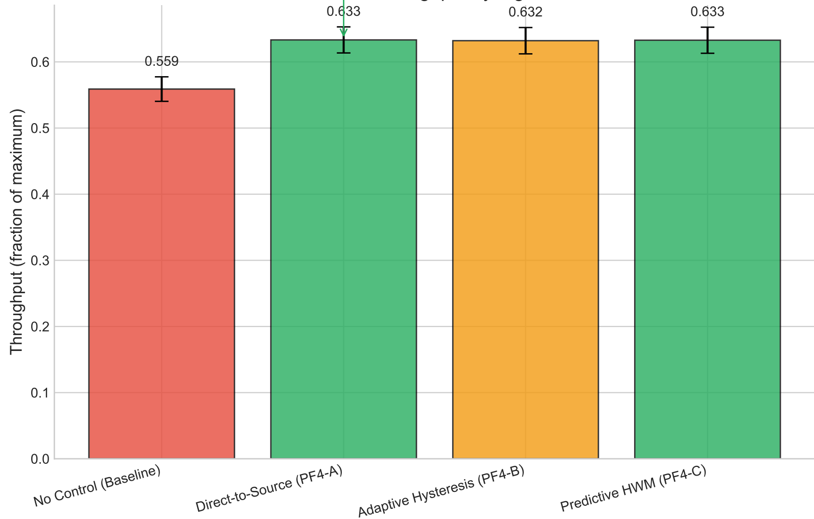
WINNER Effective Throughput by Algorithm
