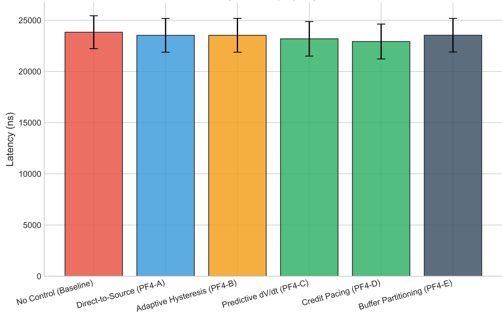
Average Latency by Algorithm
