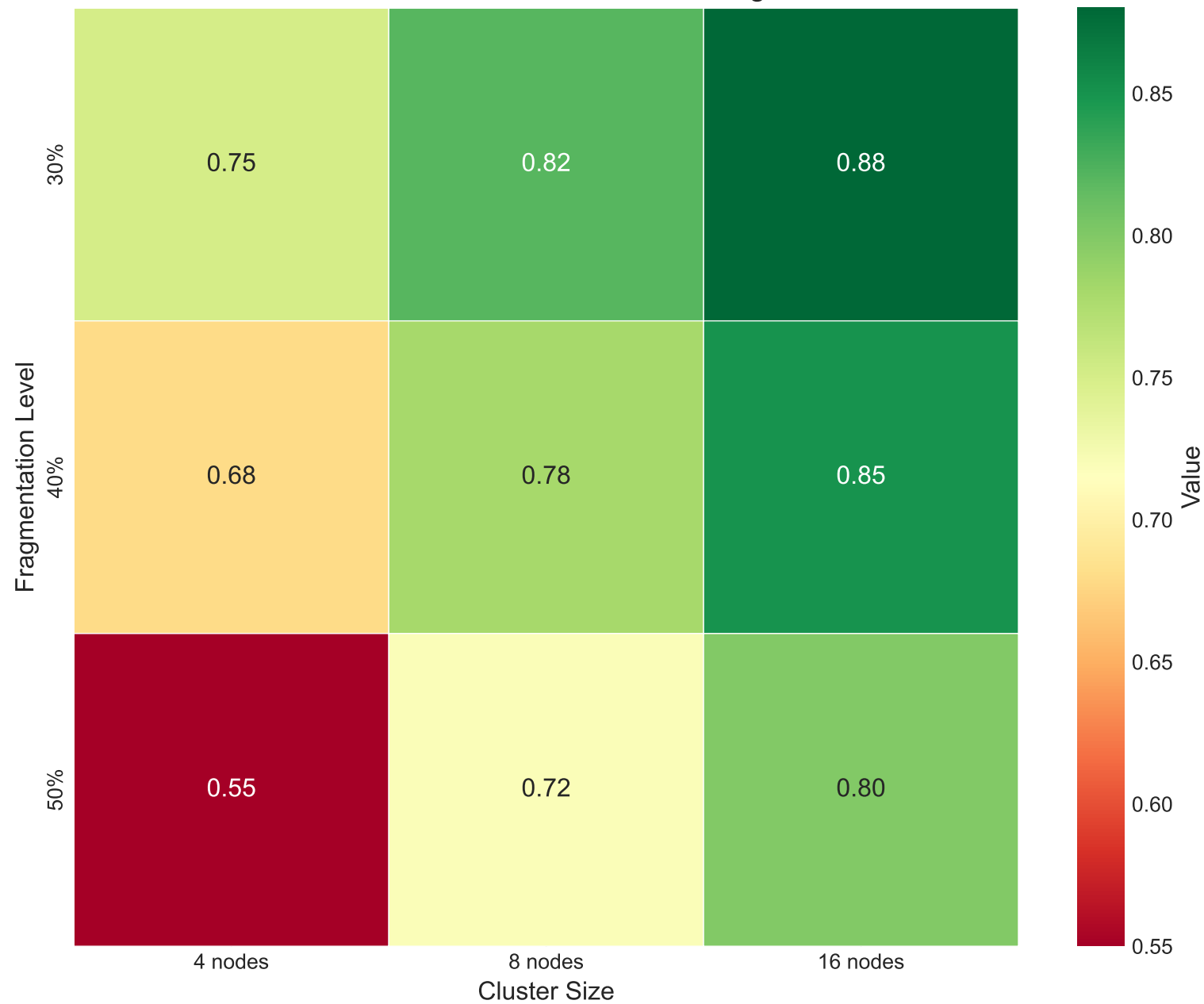
Cluster Utilization: Balanced Borrow Algorithm
