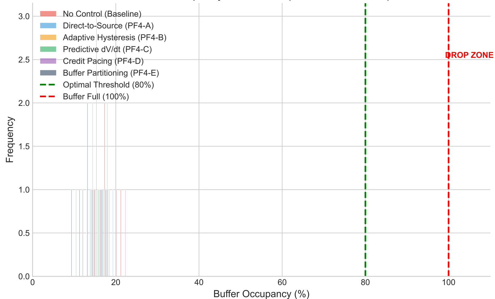
Buffer Occupancy Distribution (Incast, 50 Senders)
