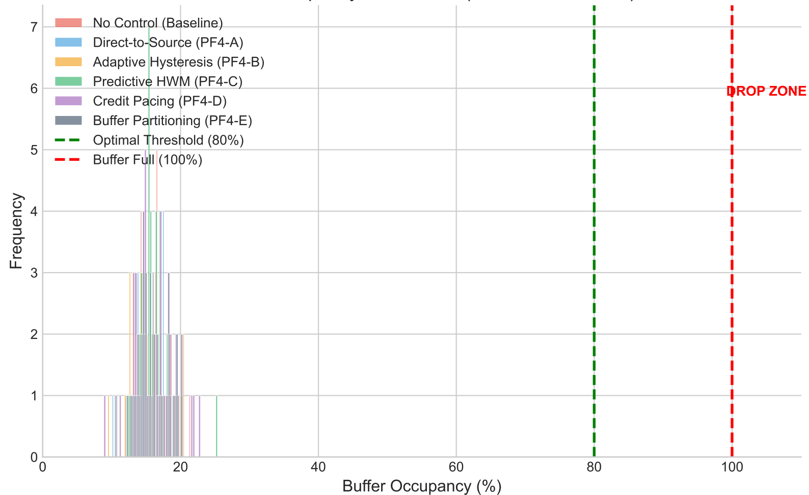
Buffer Occupancy Distribution (Incast, 50 Senders)
