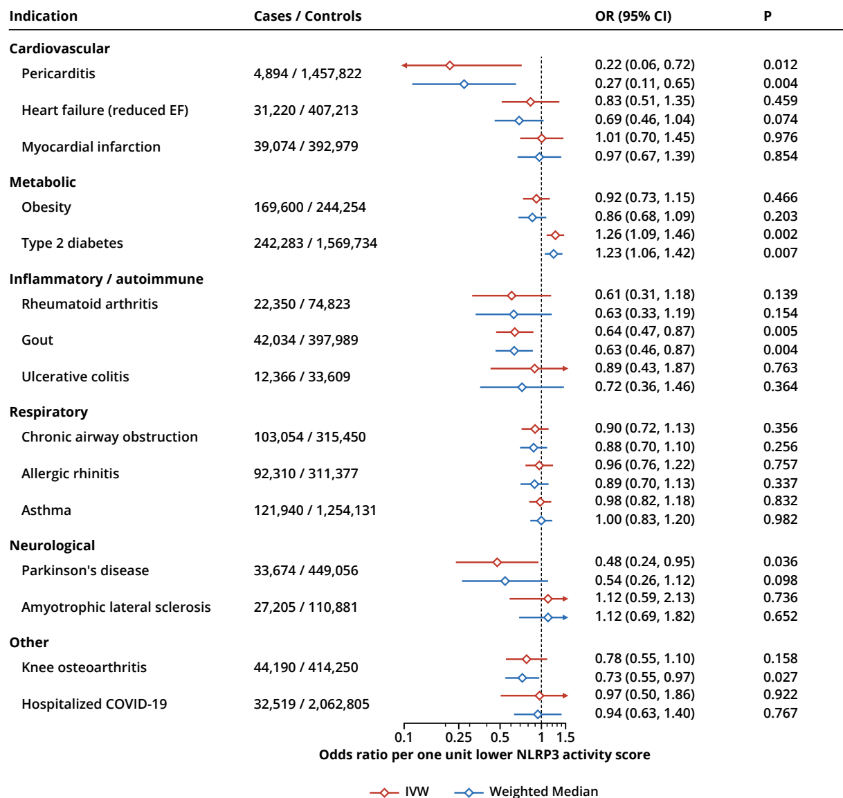
Figure 5. NLRP3 activity score associations across diseases under investigation for NLRP3 inhibition. Forest plot showing MR estimates for the association of a lower NLRP3 activity score with diseases for which NLRP3 inhibitors have been or are being evaluated in clinical trials. Outcomes are grouped by disease area. Estimates are shown as odds ratios per one-unit lower NLRP3 activity score, from inverse-variance weighted and weighted median MR. EF, ejection fraction.
