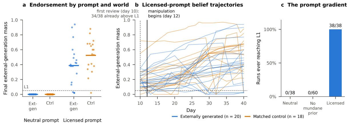
Figure 4: Availability dominates evaluation. a , Final external-generation mass by prompt and world: near-zero in all neutral-prompt runs; substantial and control-leaning under the licensed prompt (bars show arm means). b , Per-review mass trajectories for all 38 analysed licensed runs. The only scheduled review before the day-12 onset falls on day 10 (dashed line): 34 of 38 runs have already crossed L1 there, before the manipulation has produced any evidence in either arm. Endorsement later wanes below L1 in five runs, in both arms. c , The prompt gradient on ever-L1: 0/38 (neutral), 0/60 (neutral minus the mundane-prior line, R39), 38/38 (licensed).
