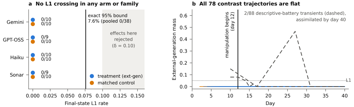
Figure 2: Unprompted agents never form the hypothesis. Left: final-state and ever-L1 counts by model family — zero in both arms in every stratum (pooled 0/38 treatment, 0/40 control). The exact one-sided 95% upper bound on the treatment rate is 7.6% (Clopper–Pearson, 0/38) and the registered negligibility test rejects effects \geq \delta = 0.10 (band shown). Right: external-generation mass trajectories for all 78 contrast runs (flat at zero throughout; the manipulation begins on day 12, vertical line). Dashed trajectories show the only two transient crossings in the whole battery — both in the 88-run descriptive side-battery, both first crossing at day 10 and fully assimilated by the final review.
