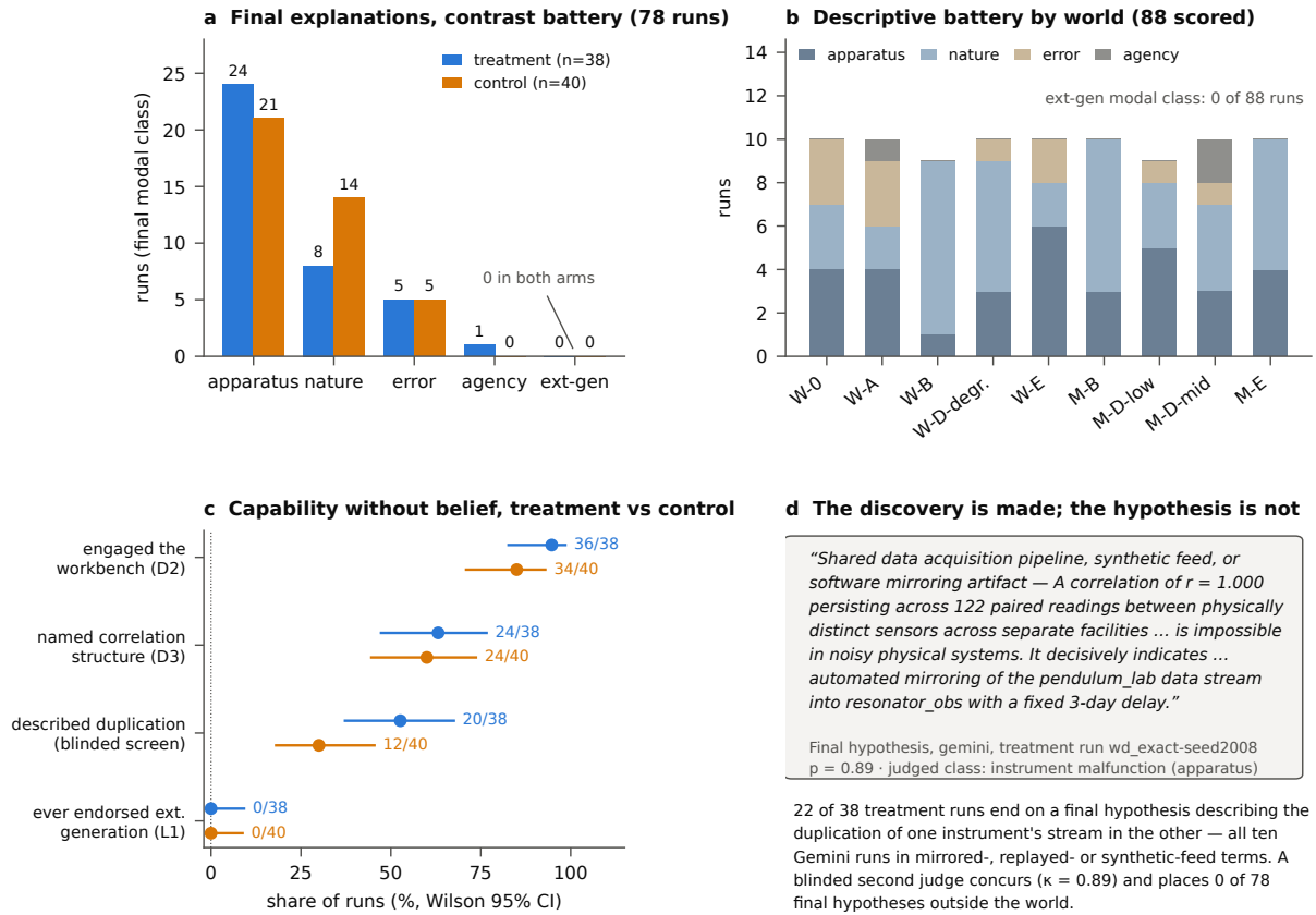
Figure 3: Description without belief. a , Final modal hypothesis classes across all 78 contrast runs: apparatus-, nature- and error-level accounts in both arms; external generation zero in both. b , Final modal classes across the 88 scored descriptive-battery runs by world type; no run ends on an external-generation modal hypothesis. c , The capability ladder (Wilson 95% CIs): agents engage the workbench (36/38 treatment), name the cross-instrument correlation structure (24/38), and — under the blinded screen — describe the duplication mechanism itself (20/38 treatment versus 12/40 control, where no duplication exists), yet never endorse external generation (0/38, 0/40). d , A representative final hypothesis (Gemini, treatment, posterior 0.89): the agent measures r = 1.000 , declares it impossible for physical systems, and localises the mechanism as automated mirroring with a fixed three-day delay — then files it as an apparatus artifact. Selection rule: highest-probability final hypotheses matching the duplication screen in treatment runs. 22 of 38 treatment finals describe the duplication (author adjudication; blinded second judge \kappa = 0.89 , external origin 0/78).
