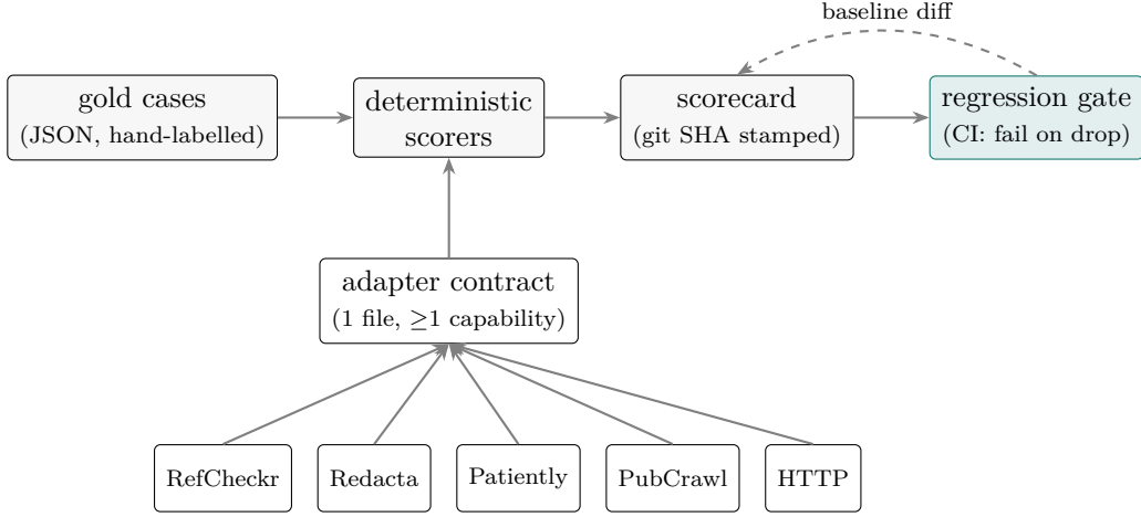
Figure 1: Gold cases and deterministic scorers produce a SHA-stamped scorecard, which is diffed against a committed per-adapter baseline; any drop in a rate metric fails the build. Systems under test attach through a one-file adapter, so the same scorers evaluate four differently shaped products, plus any REST-backed system, via the configuration-driven HTTP adapter, without code.
