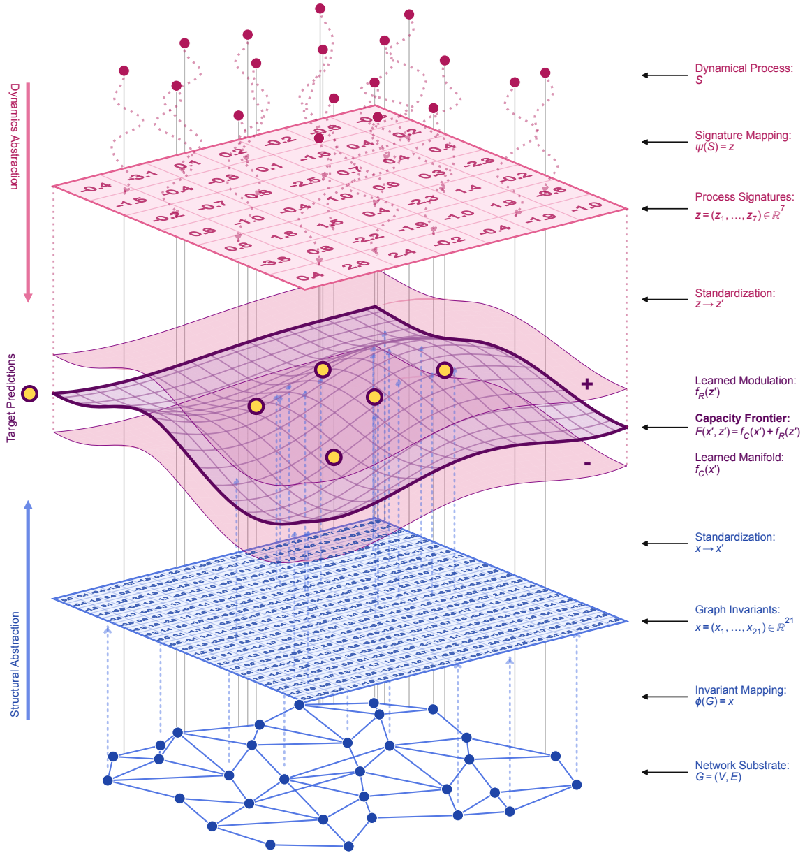
Figure 1: Conceptual representation of Structural Capacity Theory (SCT) . Schematic illustration of the Network Substrate Structured Systems (N3S). The network substrate G (blue graph, bottom) is encoded as a standardized graph invariant vector x' on the structural plane. The dynamical process S (pink markers, top) produces observations attributed to network substrate elements and is encoded as a standardized process signature vector z' on the dynamics plane. The curved manifold (purple surface, middle) represents the capacity frontier F(x', z') = f_C(x') + f_R(z') , where the learned structural component f_C(x') is modulated log-additively by the learned process component f_R(z') to estimate maximum rates y^* (gold points, middle).
