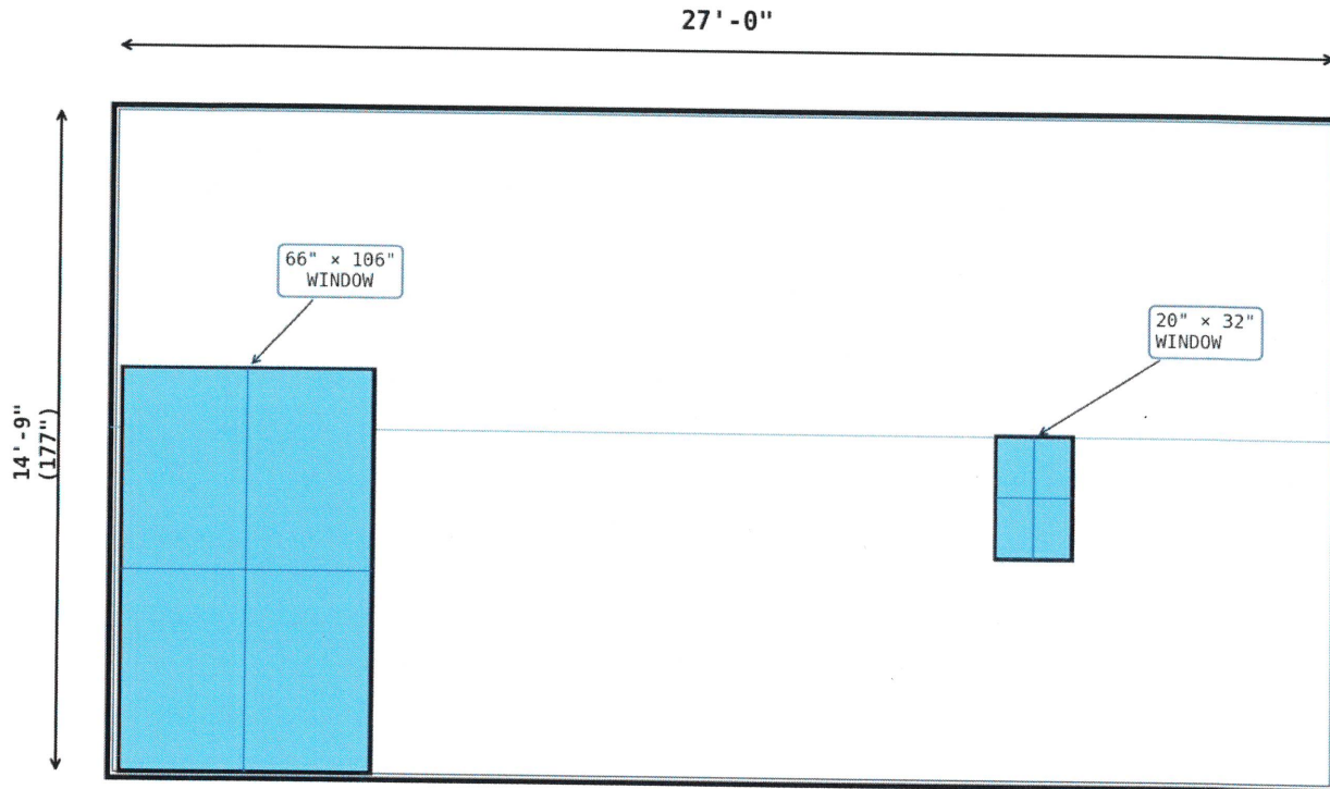
HANOVER STREET ELEVATION
