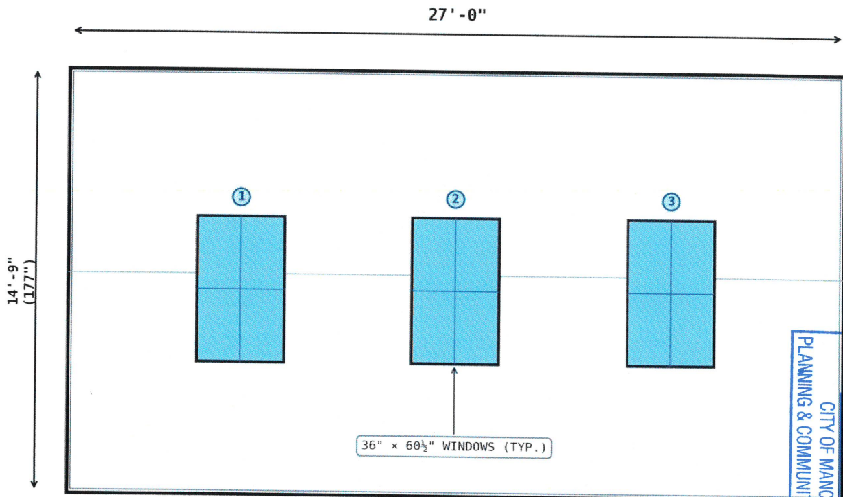
LAKE AVENUE ELEVATION
