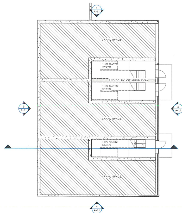
GROUND FLOOR PLAN 1/8" = 1'-0"
