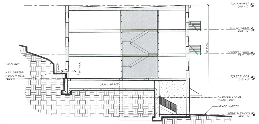
SCHEMATIC SECTION 1/8" = 1'-0"
