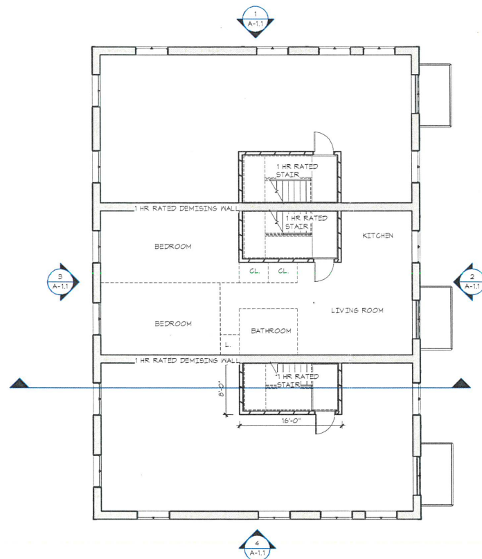
FIRST/SECOND/THIRD FLOOR PLAN 1/8" = 1'-0"
