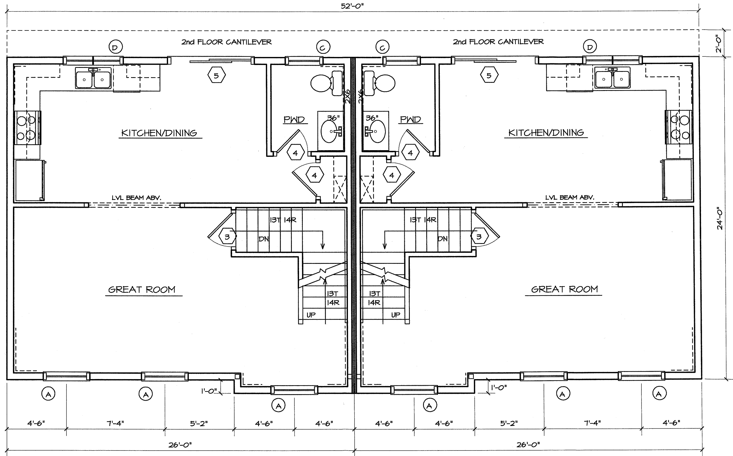
1 FIRST FLOOR PLAN A3 SCALE: 1/4" = 1'-0"
