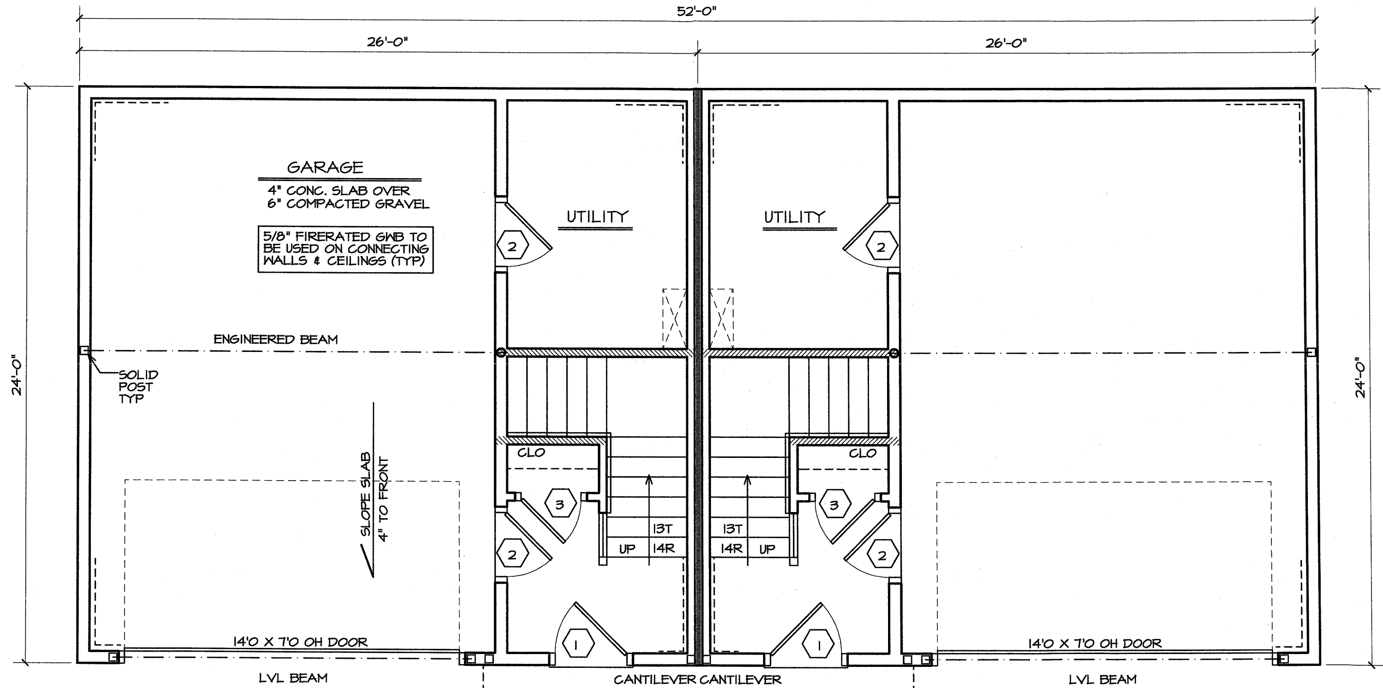
1 LOWER LEVEL PLAN A6 SCALE: 1/4" = 1'-0"
