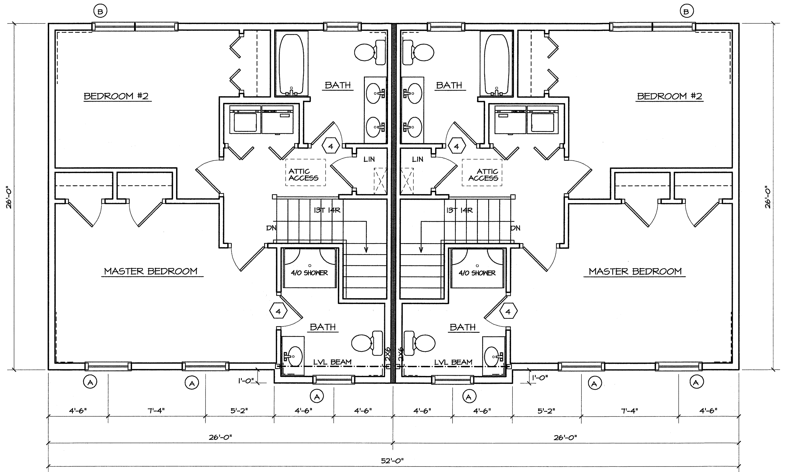
1 SECOND FLOOR PLAN A4 SCALE: 1/4" = 1'-0"
