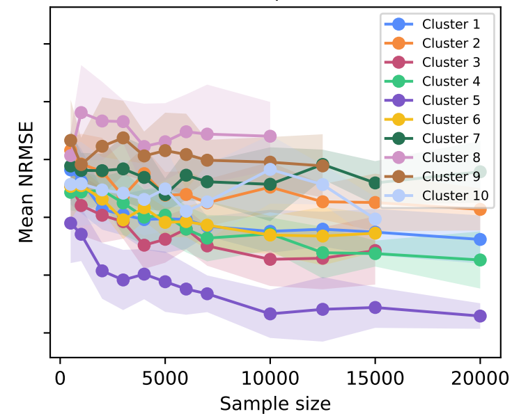
NRMSE vs sample size (k=10)
