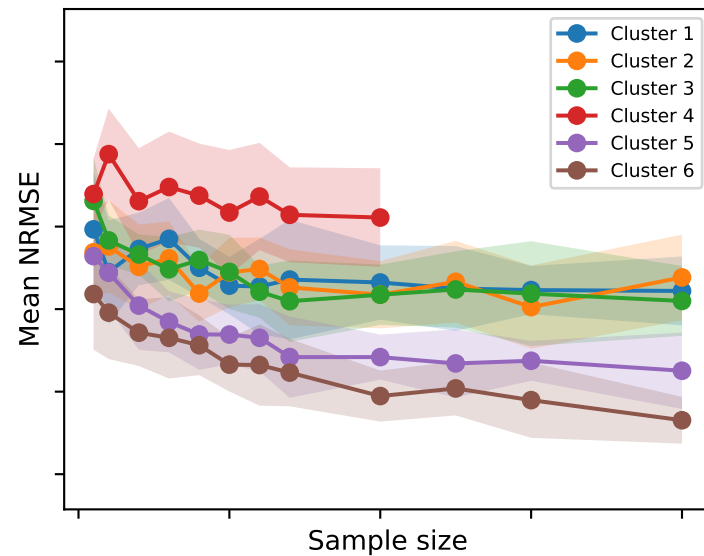
NRMSE vs sample size (k=9)
