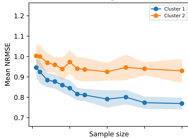
NRMSE vs sample size (k=5)
