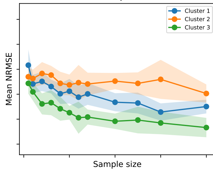
NRMSE vs sample size (k=6)
