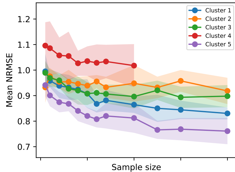
NRMSE vs sample size (k=8)
