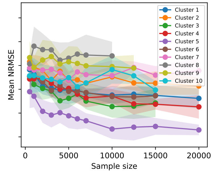
NRMSE vs sample size (k=10)
