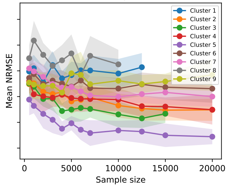
NRMSE vs sample size (k=9)
