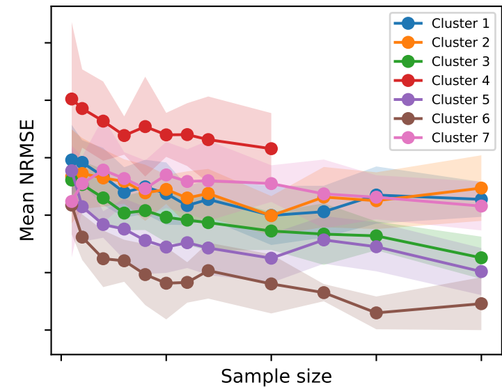
NRMSE vs sample size (k=10)
