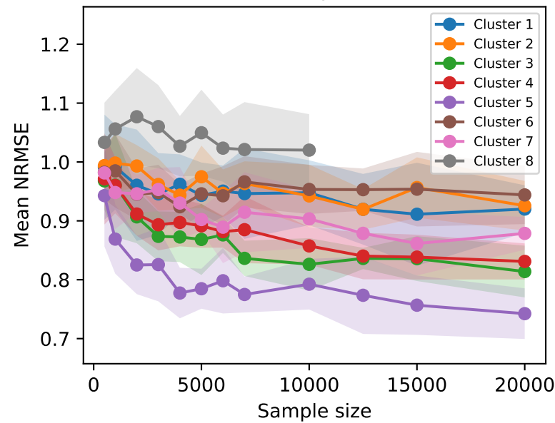
NRMSE vs sample size (k=8)
