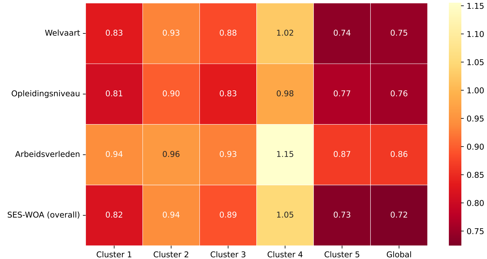
NRMSE by SES-WOA component and Cluster (5-fold CV)
