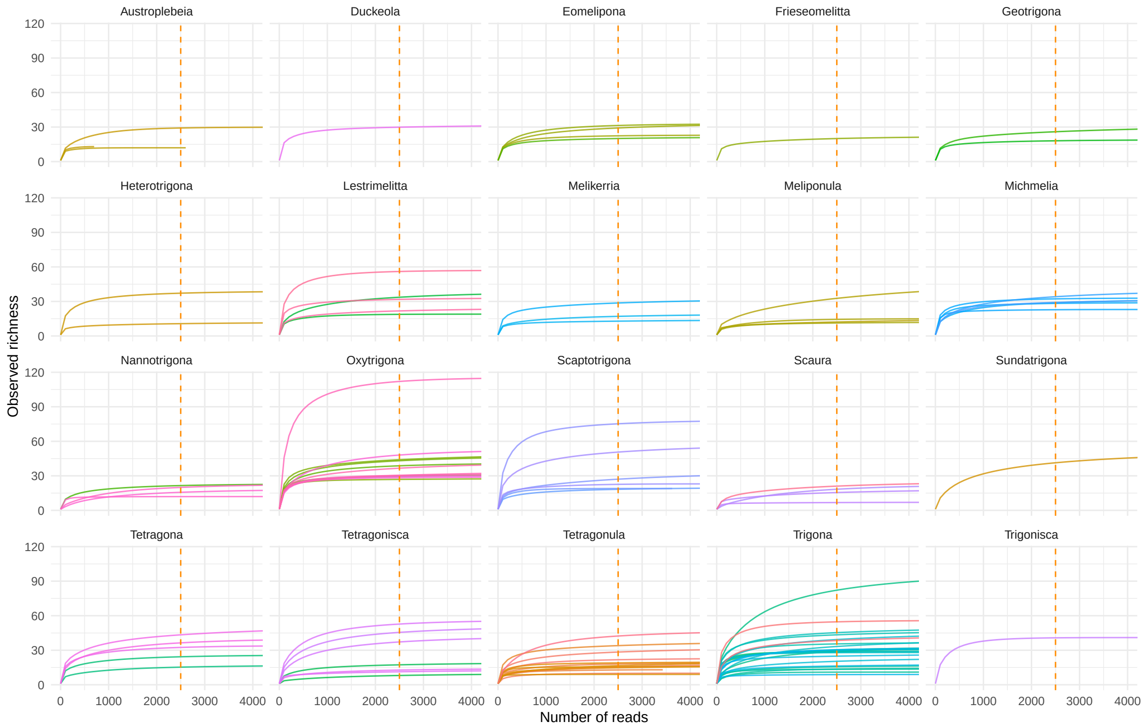
Rarefaction curves per sample (dashed line = 2,500 reads)
