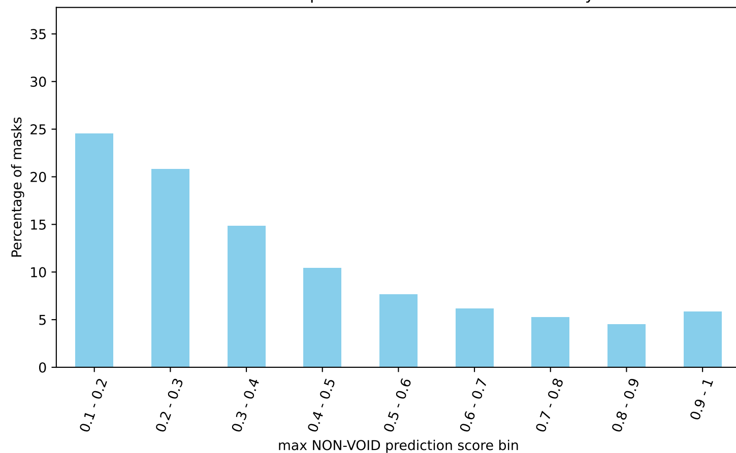
Max NON-VOID CLIP prediction score of masks correctly classified as VOID
