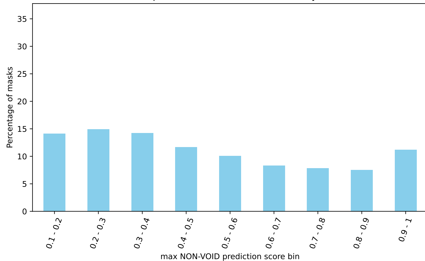
Max NON-VOID FC-CLIP prediction score of masks correctly classified as VOID
