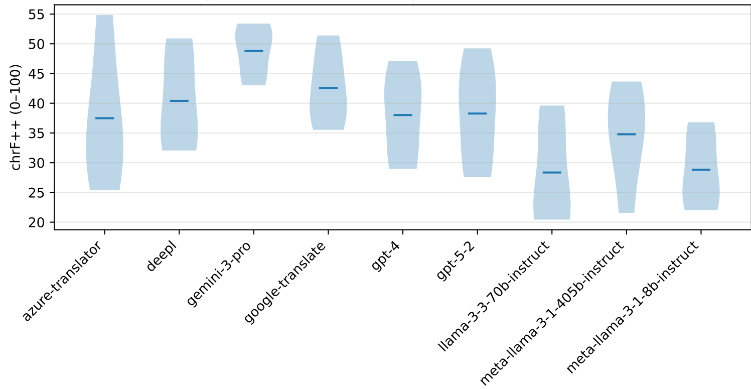
Segment-level distribution by model (chrF++) (arabic)
