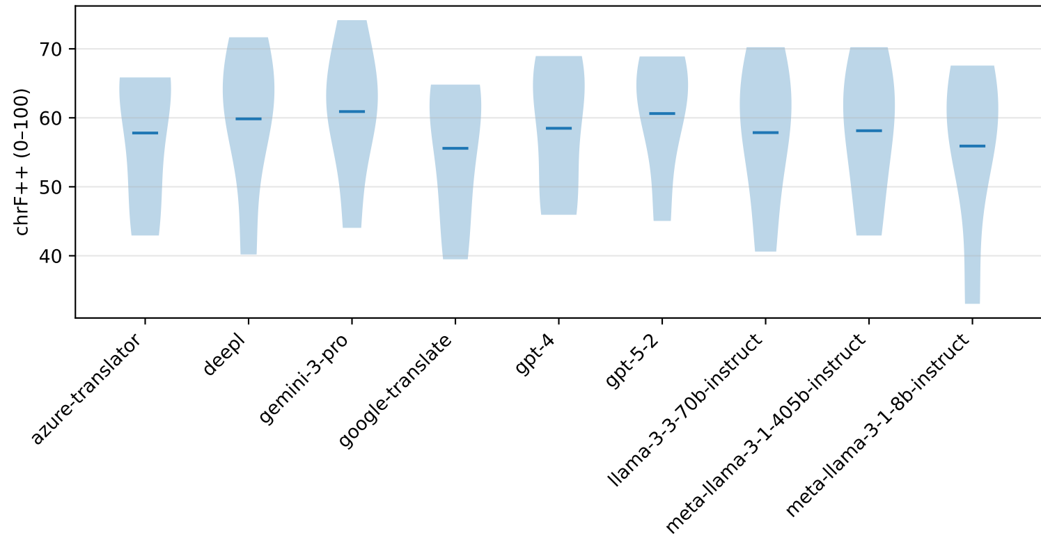
Segment-level distribution by model (chrF++) (english)
