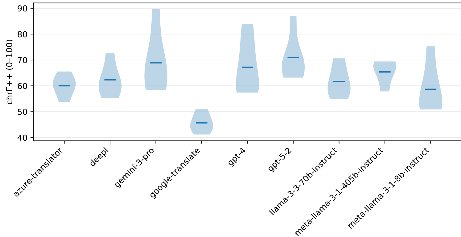
Segment-level distribution by model (chrF++) (german)
