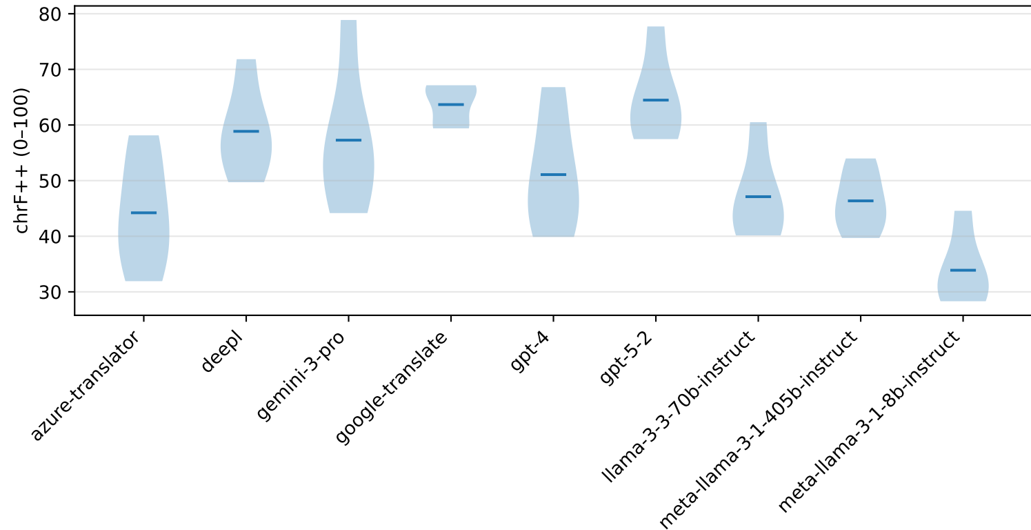
Segment-level distribution by model (chrF++) (polish)
