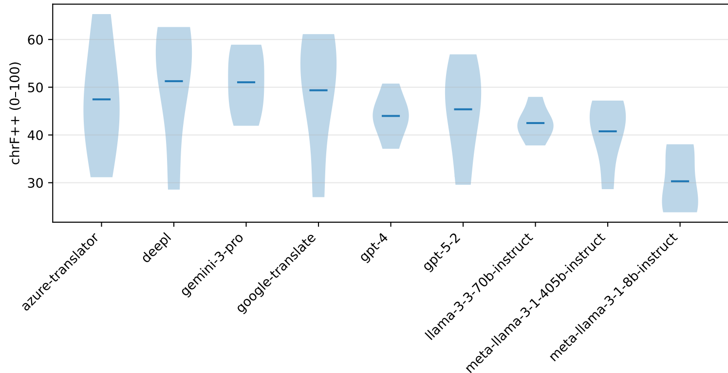
Segment-level distribution by model (chrF++) (turkish)
