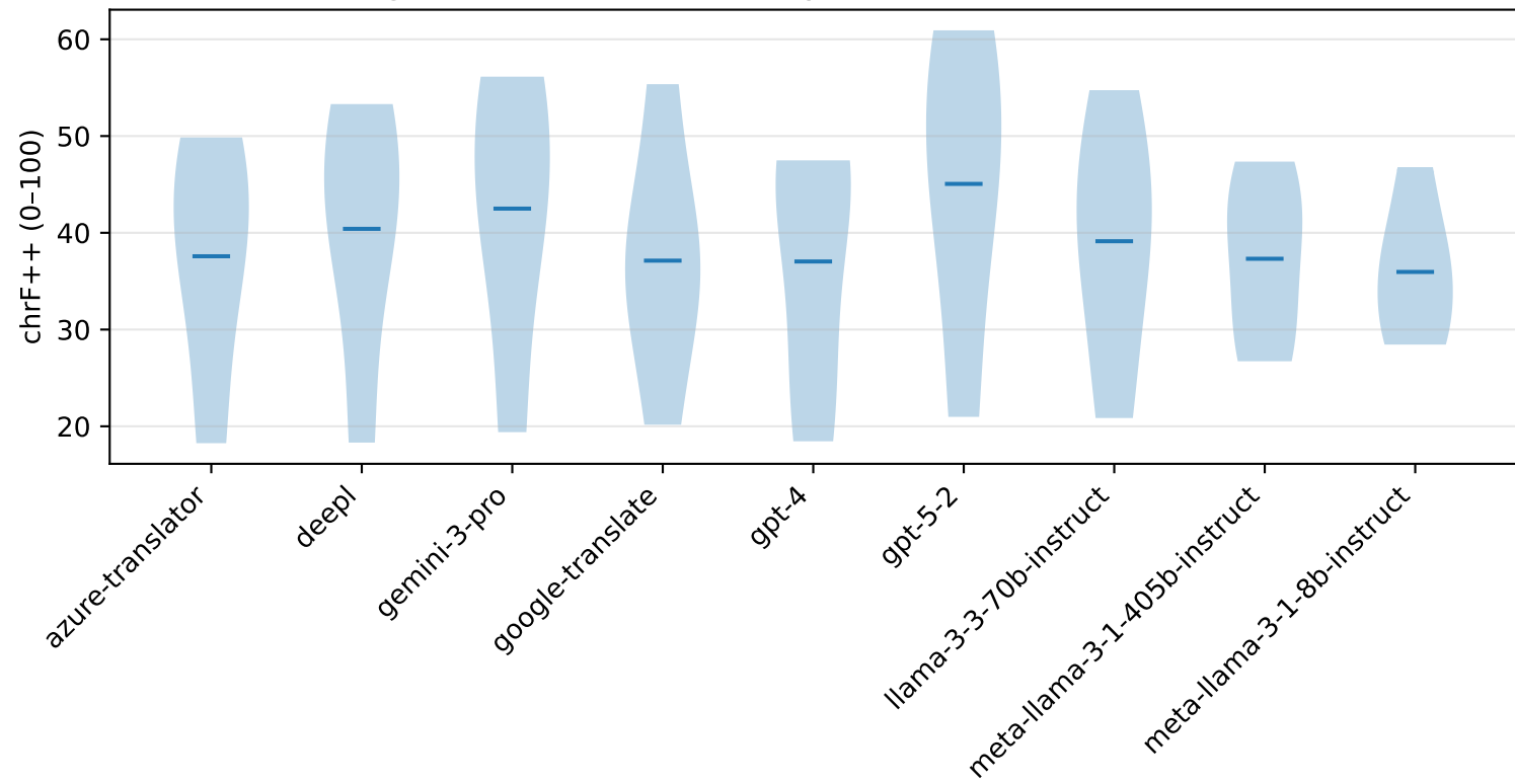
Segment-level distribution by model (chrF++) (ukrainian)
