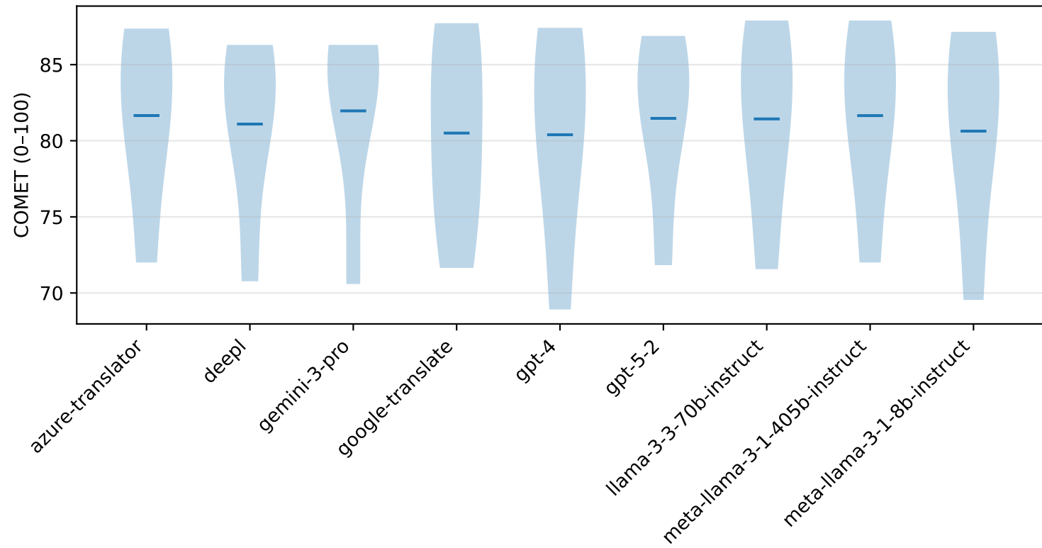
Segment-level distribution by model (COMET) (english)
