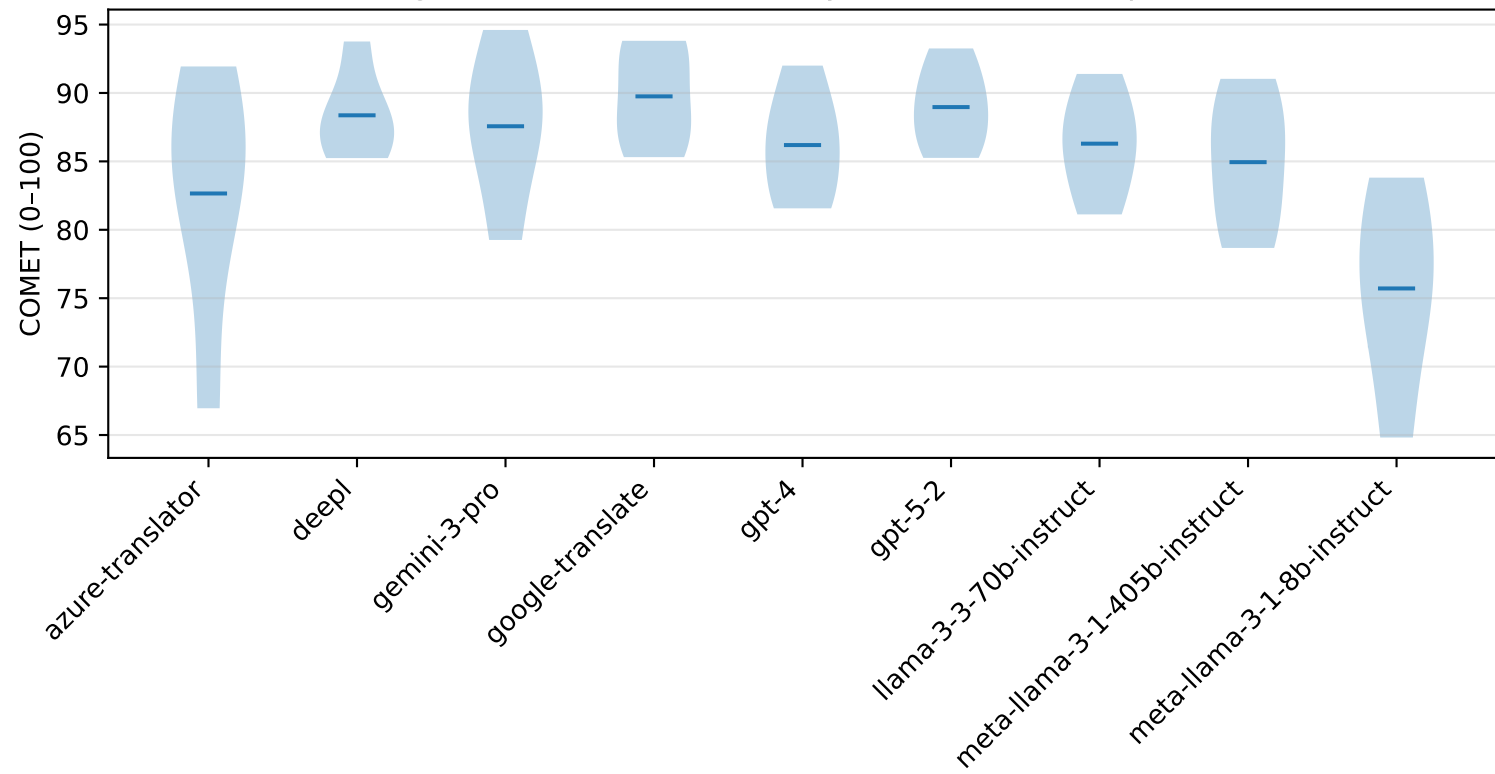
Segment-level distribution by model (COMET) (polish)
