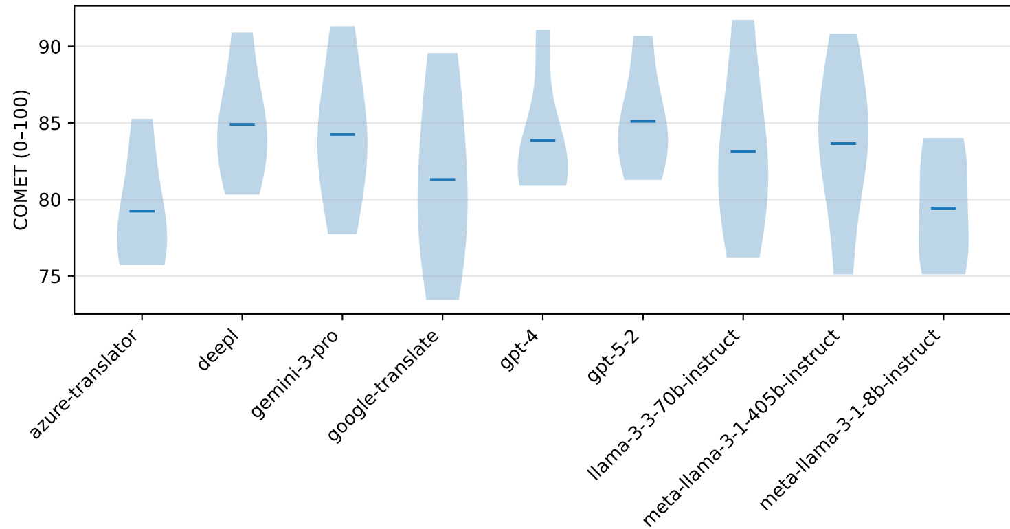
Segment-level distribution by model (COMET) (spanish)
