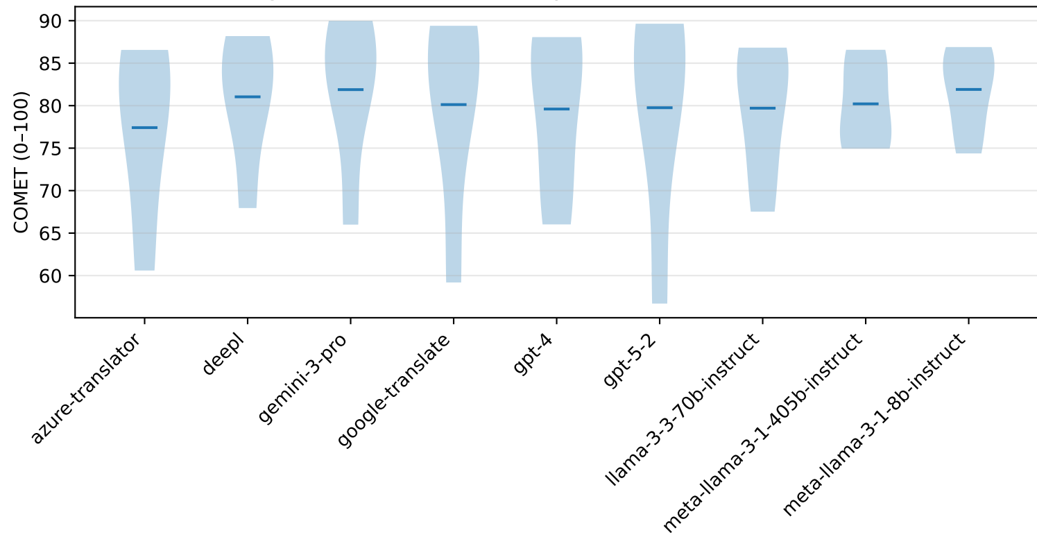
Segment-level distribution by model (COMET) (ukrainian)
