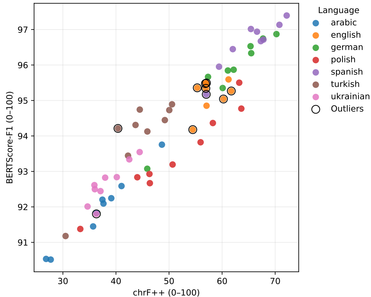
chrF++ vs BERTScore-F1
