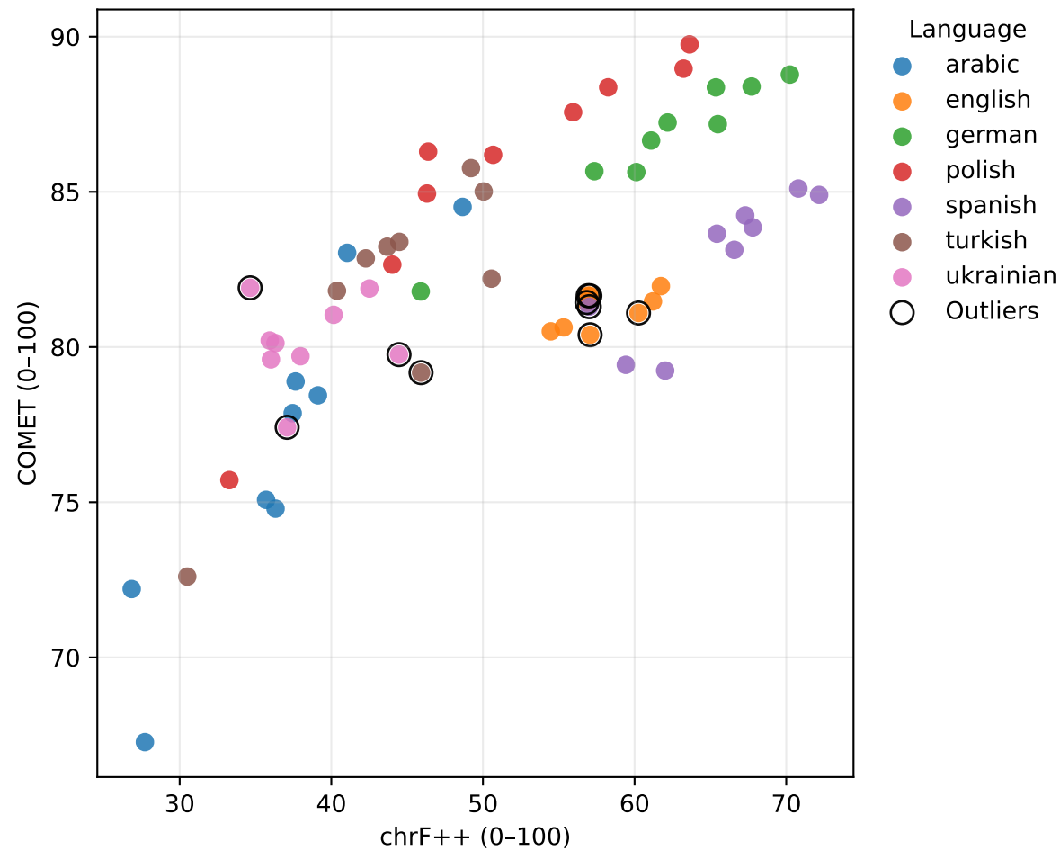
chrF++ vs COMET
