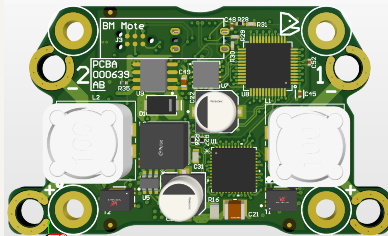
BOTTOM VIEW
