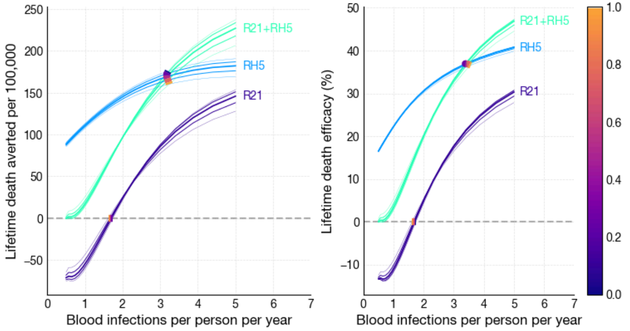
Figure 9: Blood infection rate heterogeneity, \beta = (0, 1) .
