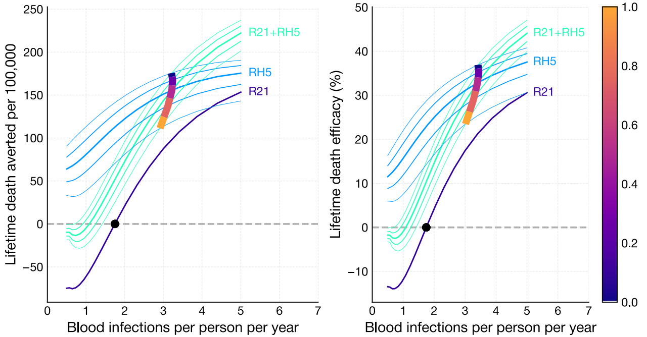
Figure 15: RH5 protective effect against blood infection, \omega_{infection} = (0, 1) .
