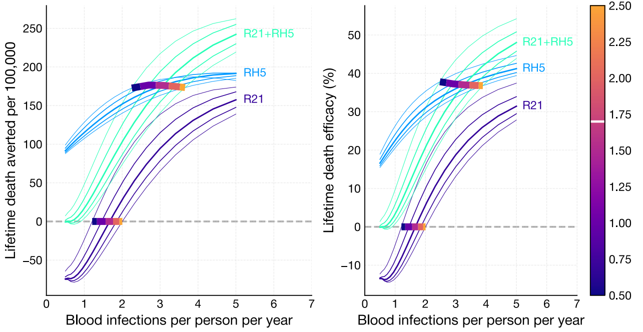
Figure 2: Half-life of early life protection from infection, \tau_{\text{elp}} = (0.5, 2.0) years.
