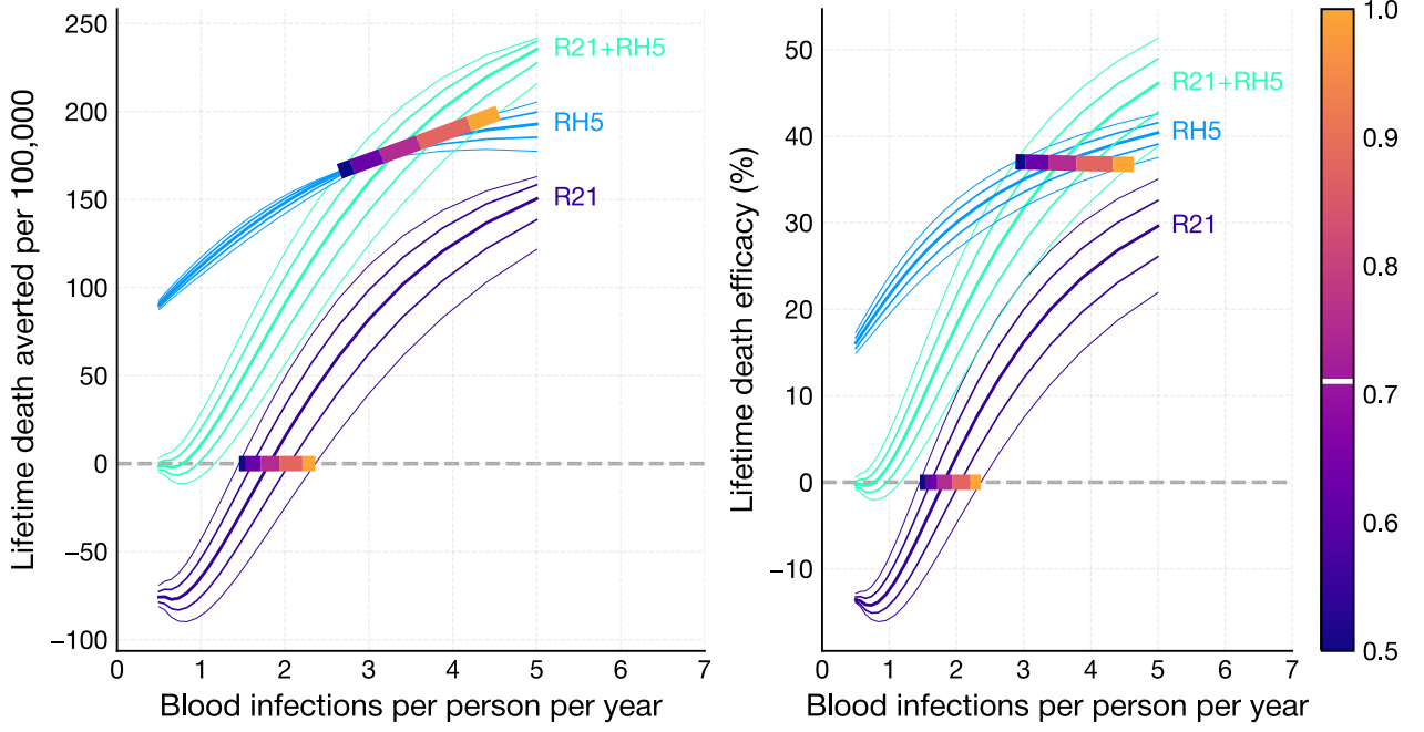
Figure 1: Early life protection from infection at birth, \rho_{\text{elp}} = (0.5, 1) . The default value is shown as a white line in the colorbar. For a given value of \rho_{\text{elp}} and for each vaccine strategy (R21-alone, RH5-alone and RH5+R21 combined, all with one booster) we run 20 simulations across the range of infection rates from 0.5 to 5 blood infections per year. The point of intersection of the R21+RH5 line and the RH5 line is the critical threshold \lambda_{\text{RH5}} . And the point of intersection of the R21 line with the x -axis is the critical threshold \lambda_{\text{R21}} . We repeat the process for five different values of \rho_{\text{elp}} equally spaced between 0.5 and 1 inclusive. The resulting five values of \lambda_{\text{RH5}} are joined by a coloured line with the colour representing the value of \rho_{\text{elp}} which is shown in the colorbar. The same is done for \lambda_{\text{R21}} . Thus the coloured lines show the sensitivity of the two critical thresholds to changes in \rho_{\text{elp}} .
