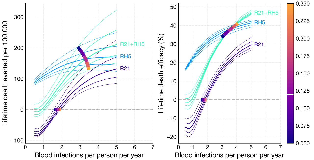
Figure 7: Rate of decline in risk of severe malaria with exposure in newborns, \delta_{\text{severe}} = (0.05, 0.25) per infection.
