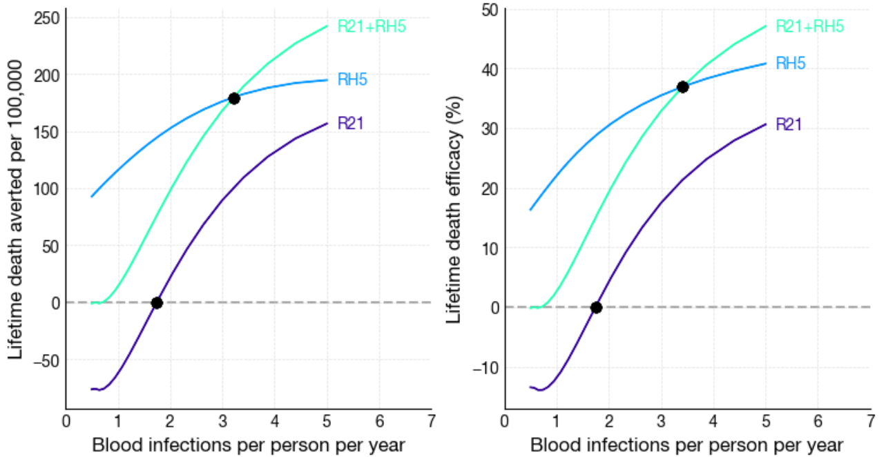
Figure 4: Half-maximum risk exposure of clinical malaria, \gamma_{\text{clinical}} = (10, 200) infections.
