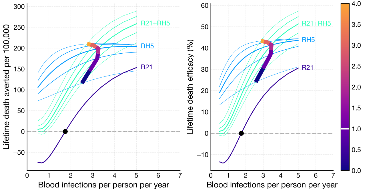
Figure 14: Number of RH5 boosters = 0, ..., 4, default 1.
