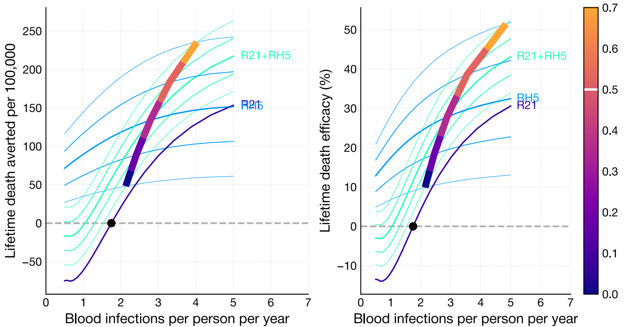
Figure 16: RH5 protective effect against clinical malaria, \omega_{clinical} = (0, 0.7) .
