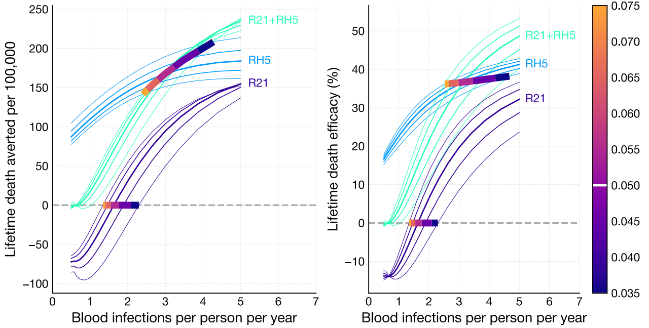
Figure 8: Age modification rate in decline in risk of severe malaria, \epsilon_{\text{severe}} = (0.035, 0.075) per infection per year.
