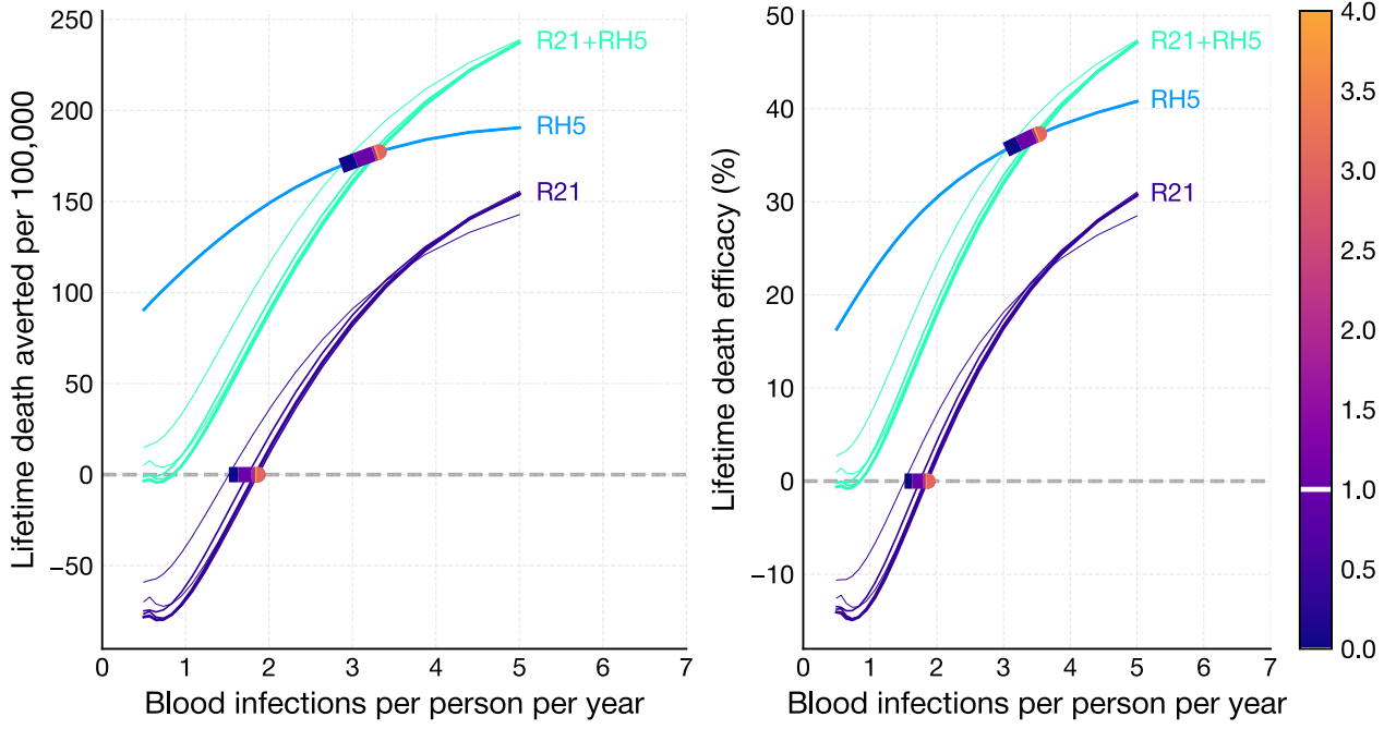
Figure 12: Number of R21 boosters = 0, ..., 4.
