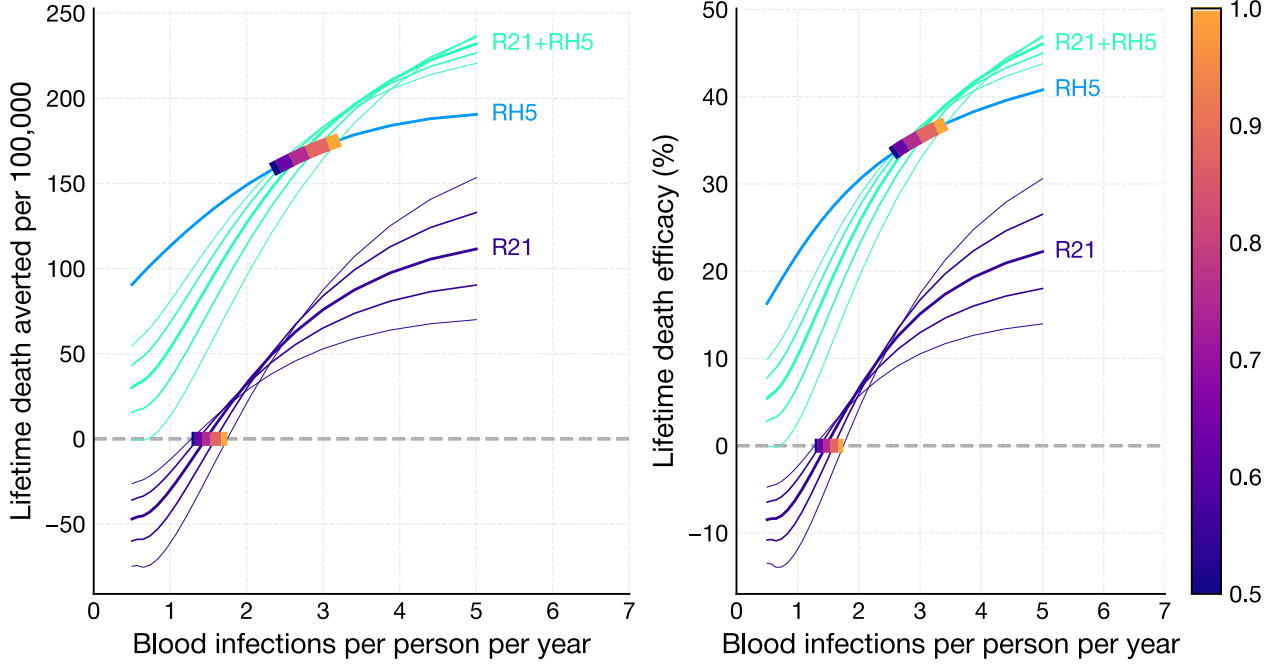
Figure 10: R21's maximum efficacy against infection, \nu_{\text{liver}} = (0.5, 1) .
