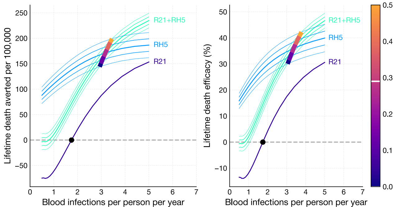
Figure 17: RH5 protective effect against severe malaria, \omega_{\text{severe}} = (0, 0.5) .
