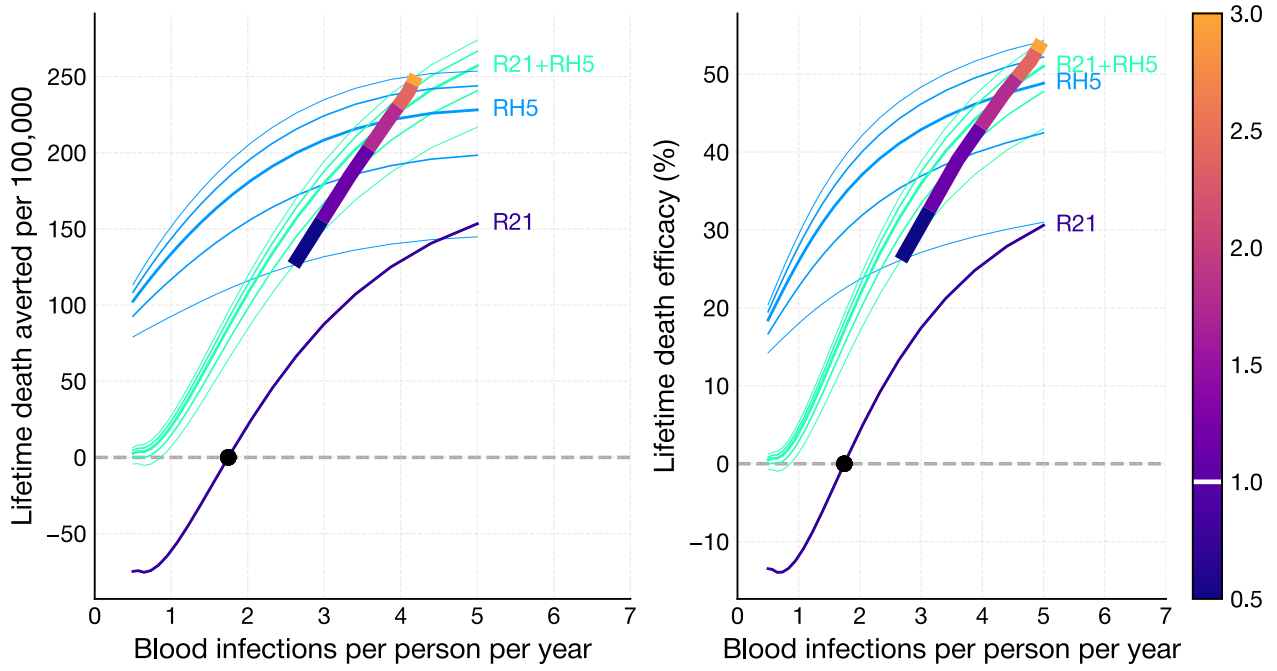
Figure 13: RH5 half-life, \tau_{\text{blood}} = (0.5, 3) default 1.
