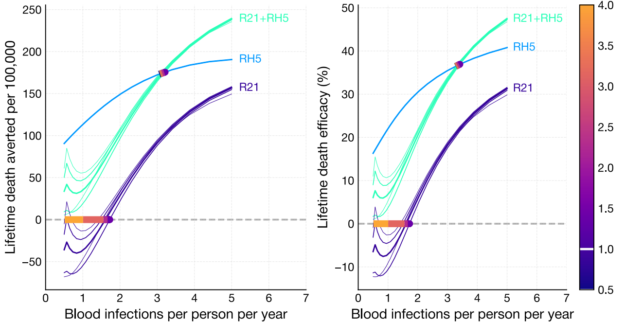
Figure 11: R21 half-life, \tau_{\text{liver}} = (0.5, 4) .
