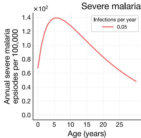
Figure 10: Model simulation for a blood infection rate of 0.05 per year recapitulates observations in Imbert et al. (1997) of severe malaria episodes persisting into adulthood.
