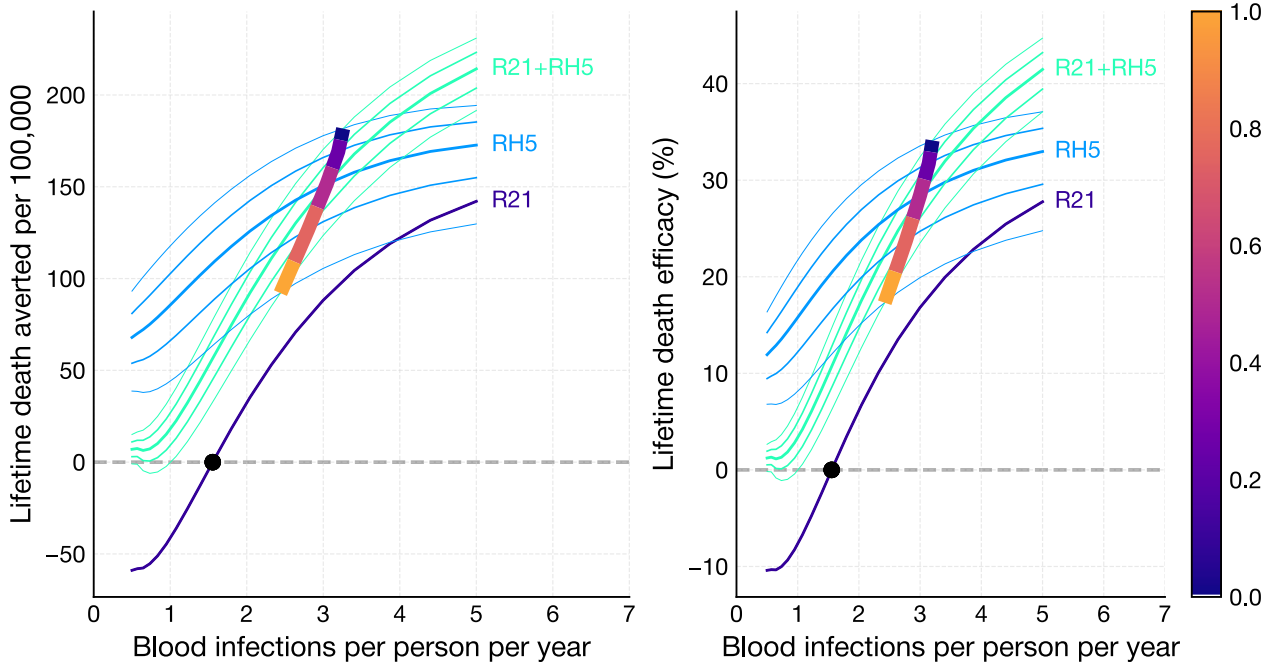
Figure 17: RH5 protective effect against blood infection, \omega_{infection} = (0, 1) .
