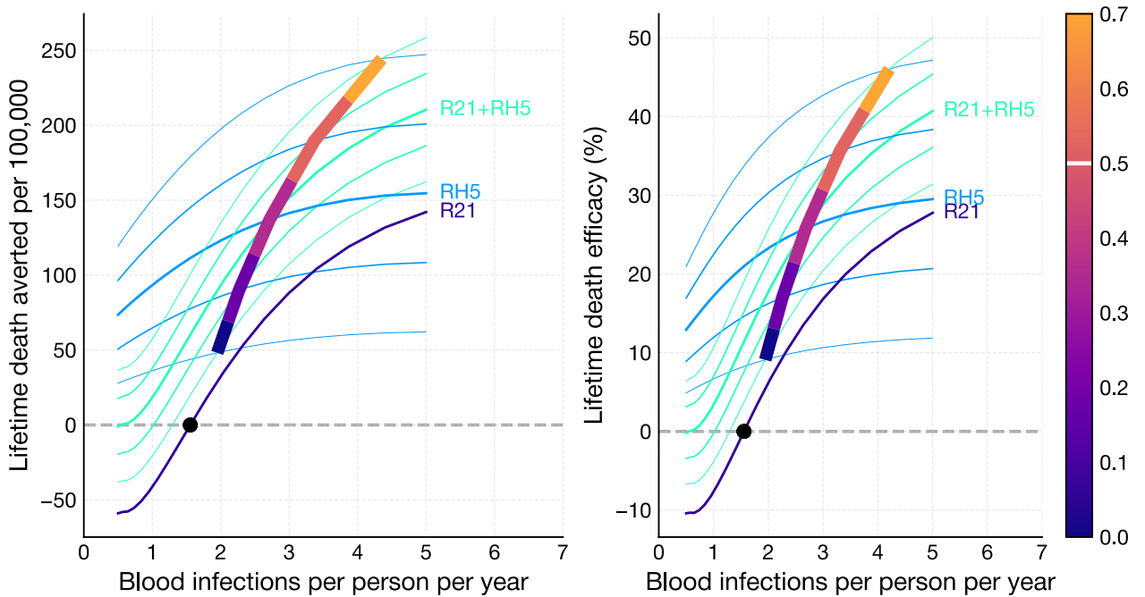
Figure 18: RH5 protective effect against clinical malaria, \omega_{clinical} = (0, 0.7) .
