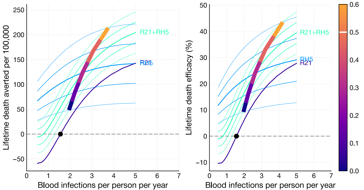
Figure 18: RH5 protective effect against clinical malaria, \omega_{\text{clinical}} = (0, 0.6) .
