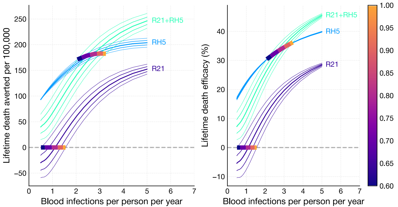
Figure 10: Attenuation of severe malaria-associated age-specific risk of death, death_rate_modifier = (0.6, 1).
