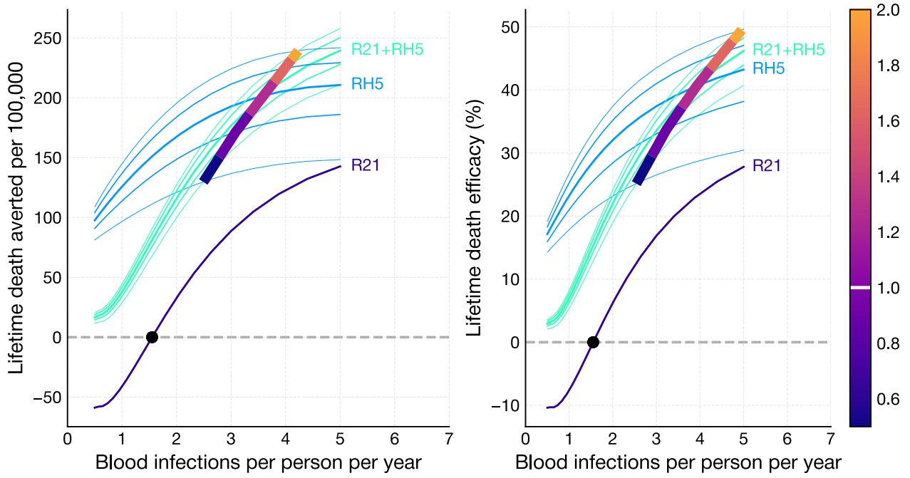
Figure 15: RH5 half-life, \tau_{\text{blood}} = (0.5, 2) default 1.
