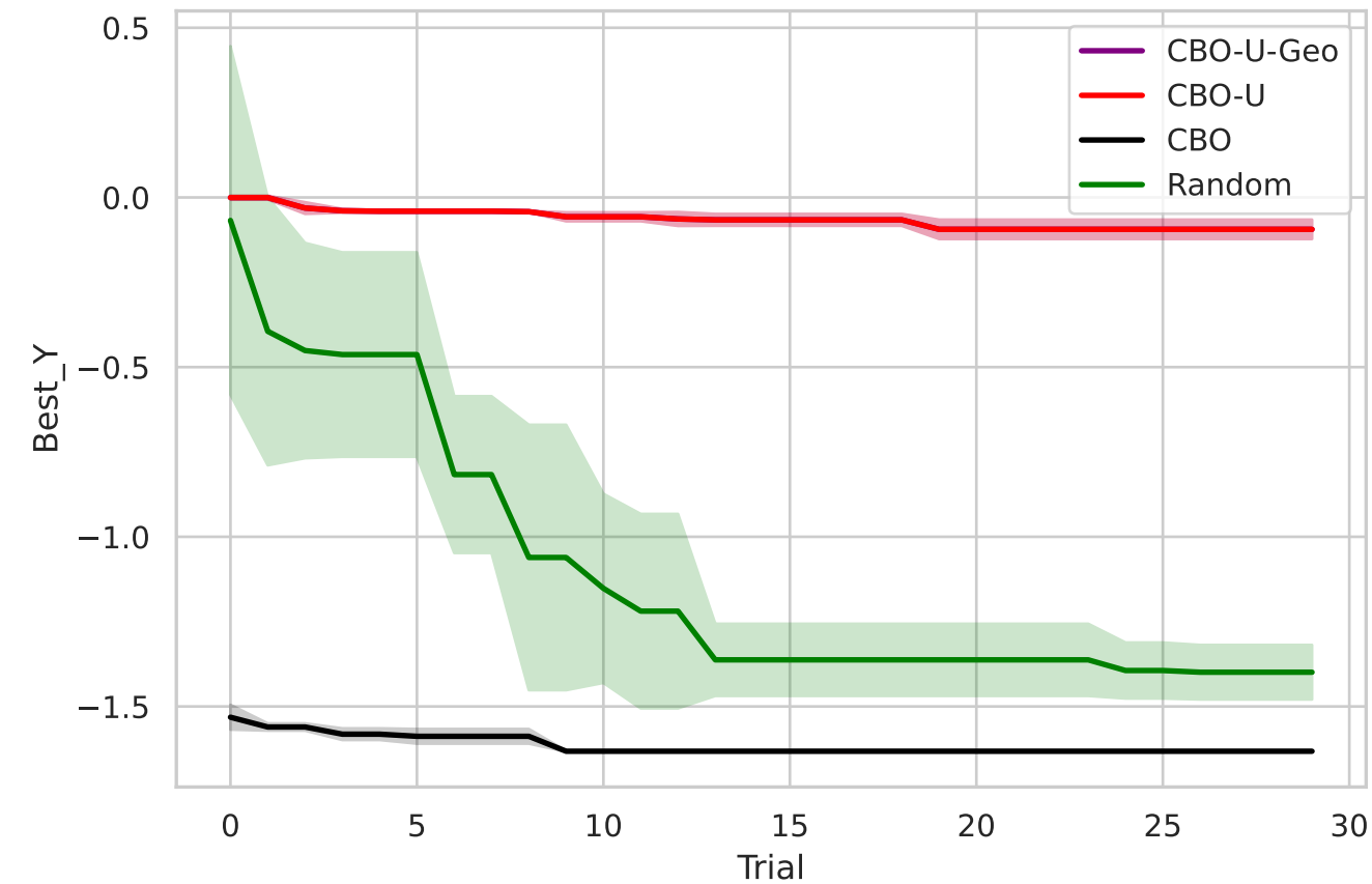
Erdos100 (linear)
