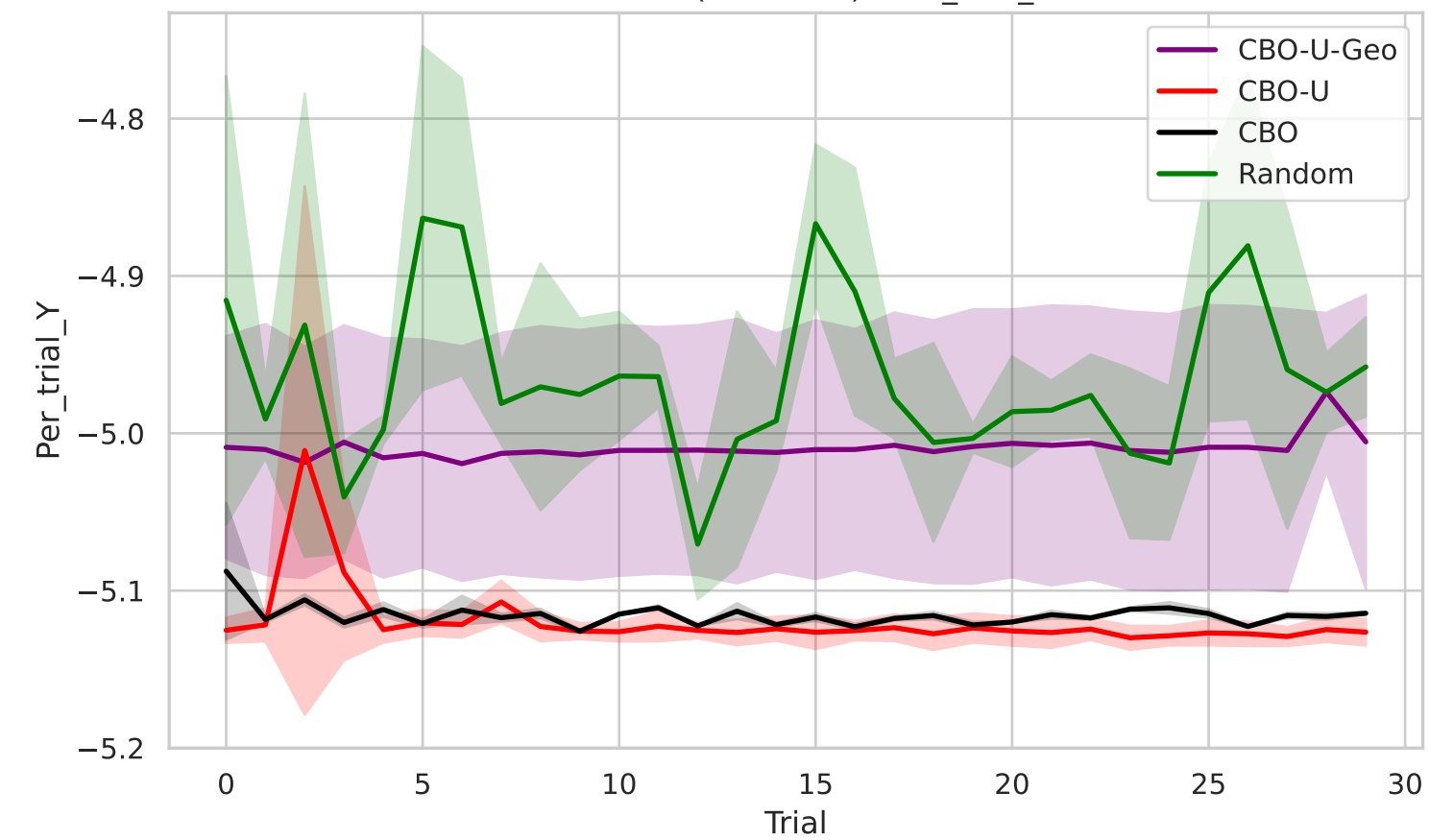
Erdos100 (nonlinear) - Per_trial_Y
