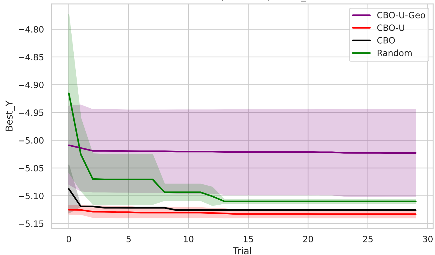
Erdos100 (nonlinear) - Best_Y
