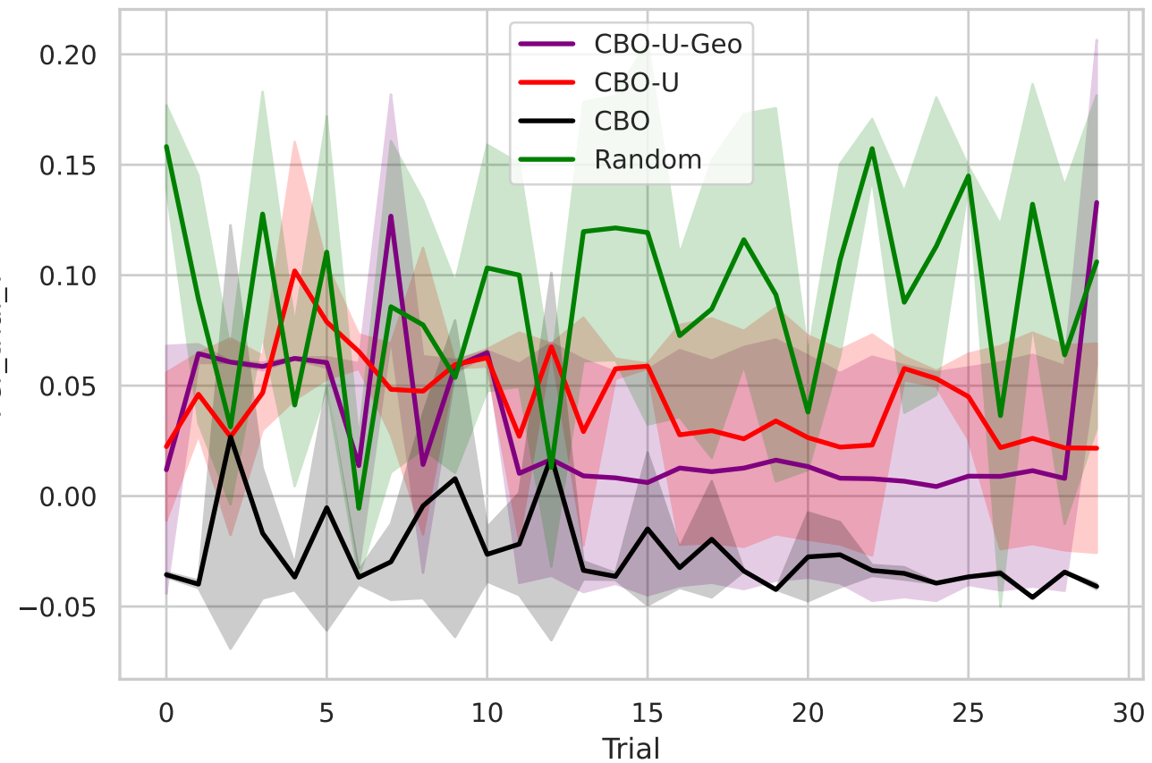
Erdos20 (nonlinear)
