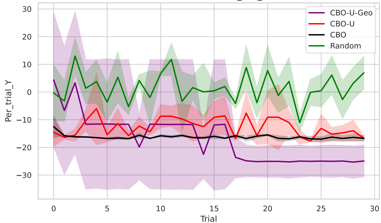
Erdos50 (linear) - Per_trial_Y
