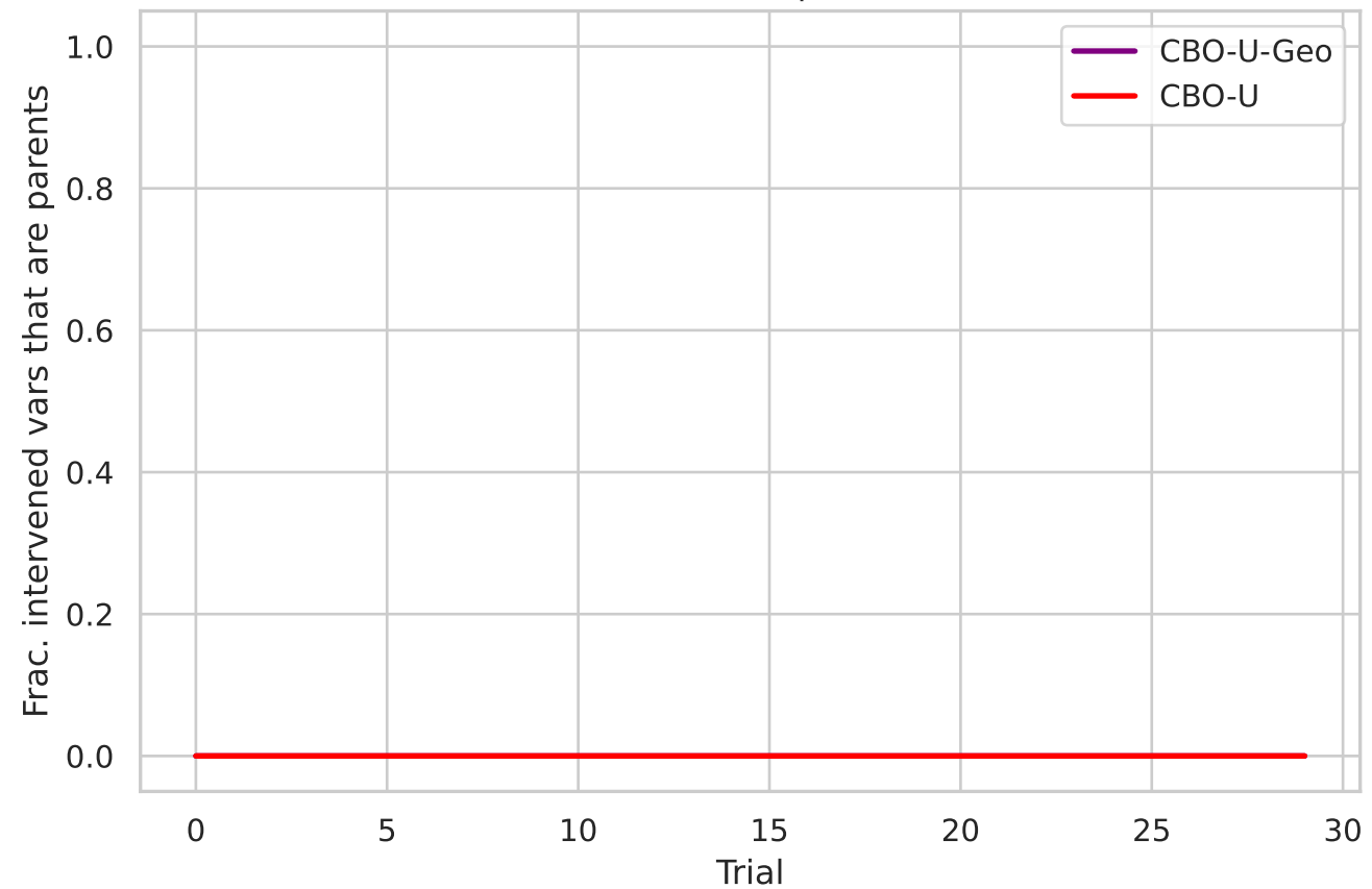
Erdos100 (linear) - true parents ['85', '98']
