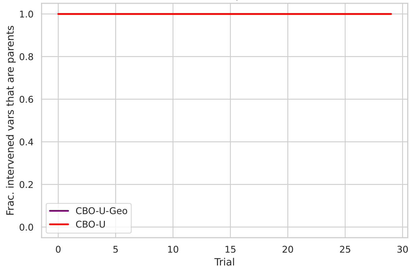
Erdos50 (linear) - true parents ['19', '49']
