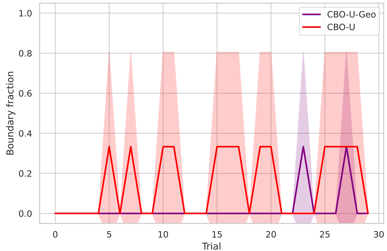
Erdos100 (linear)
