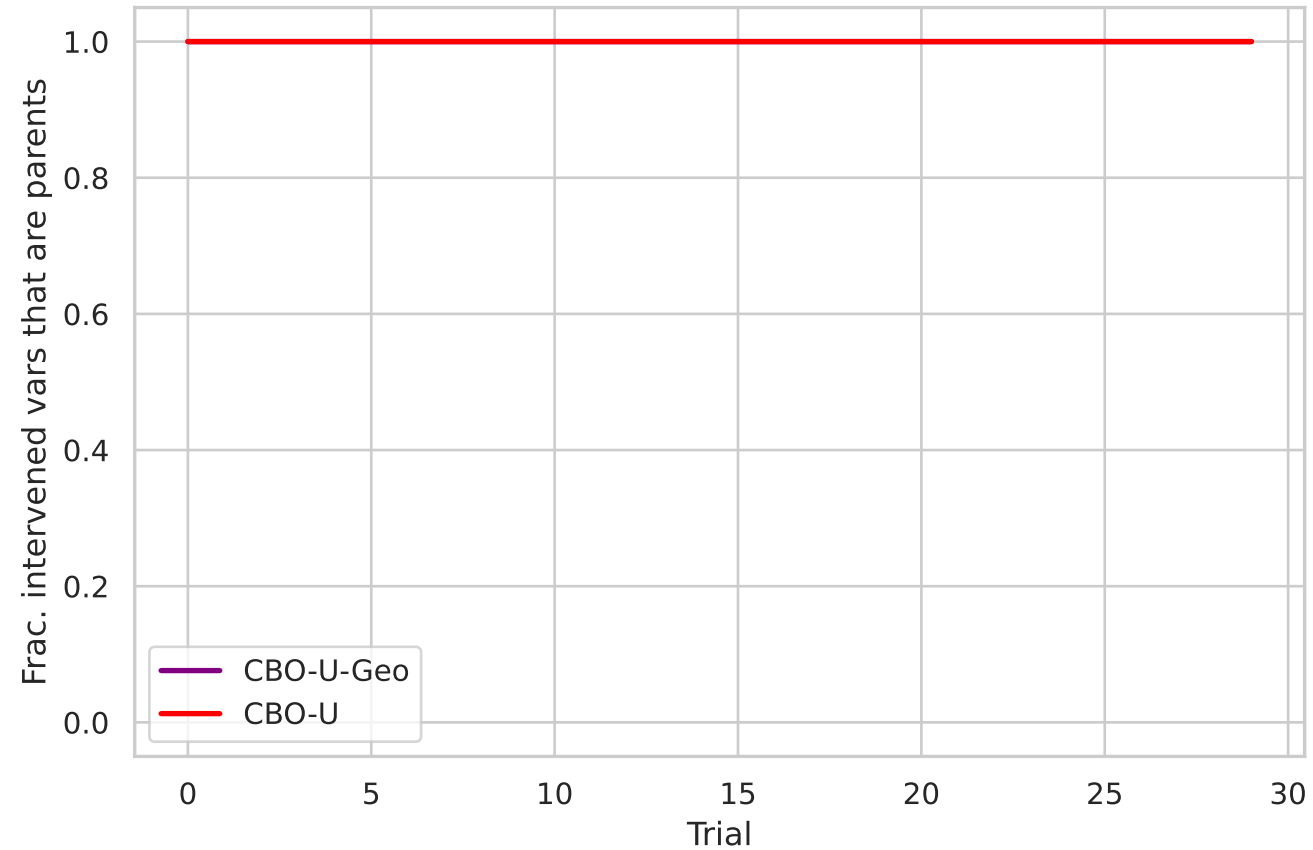
Dream100 - true parents ['4', '40', '42', '48', '78']
