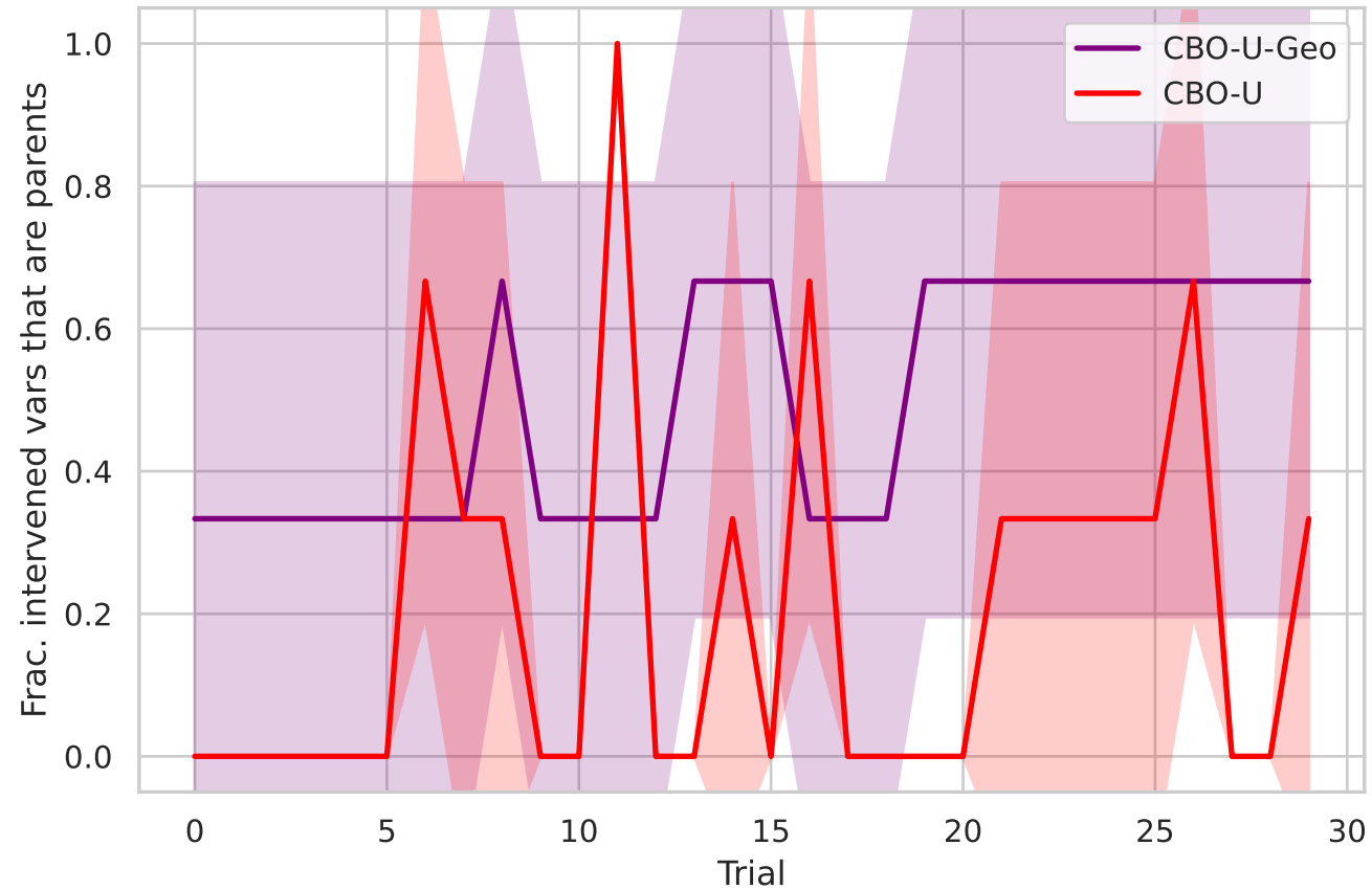
Dream50 - true parents ['3', '18', '20', '22', '23']
