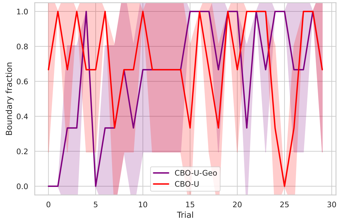
Erdos50 (nonlinear)
