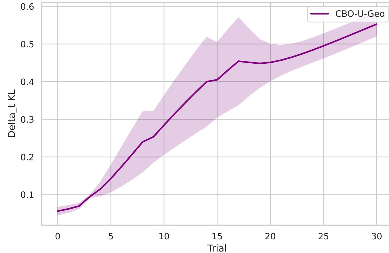
Erdos50 (linear)
