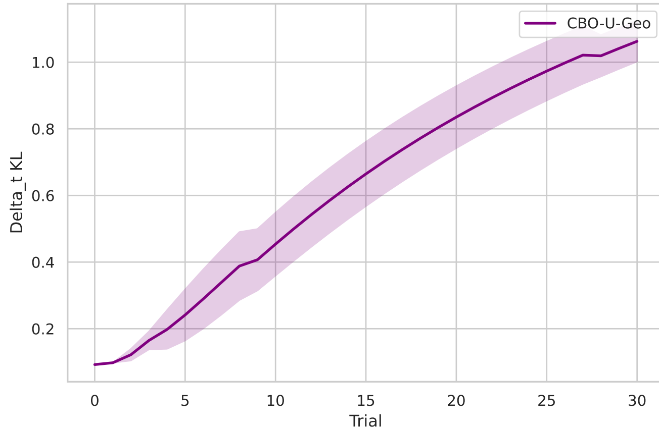
Erdos20 (linear)
